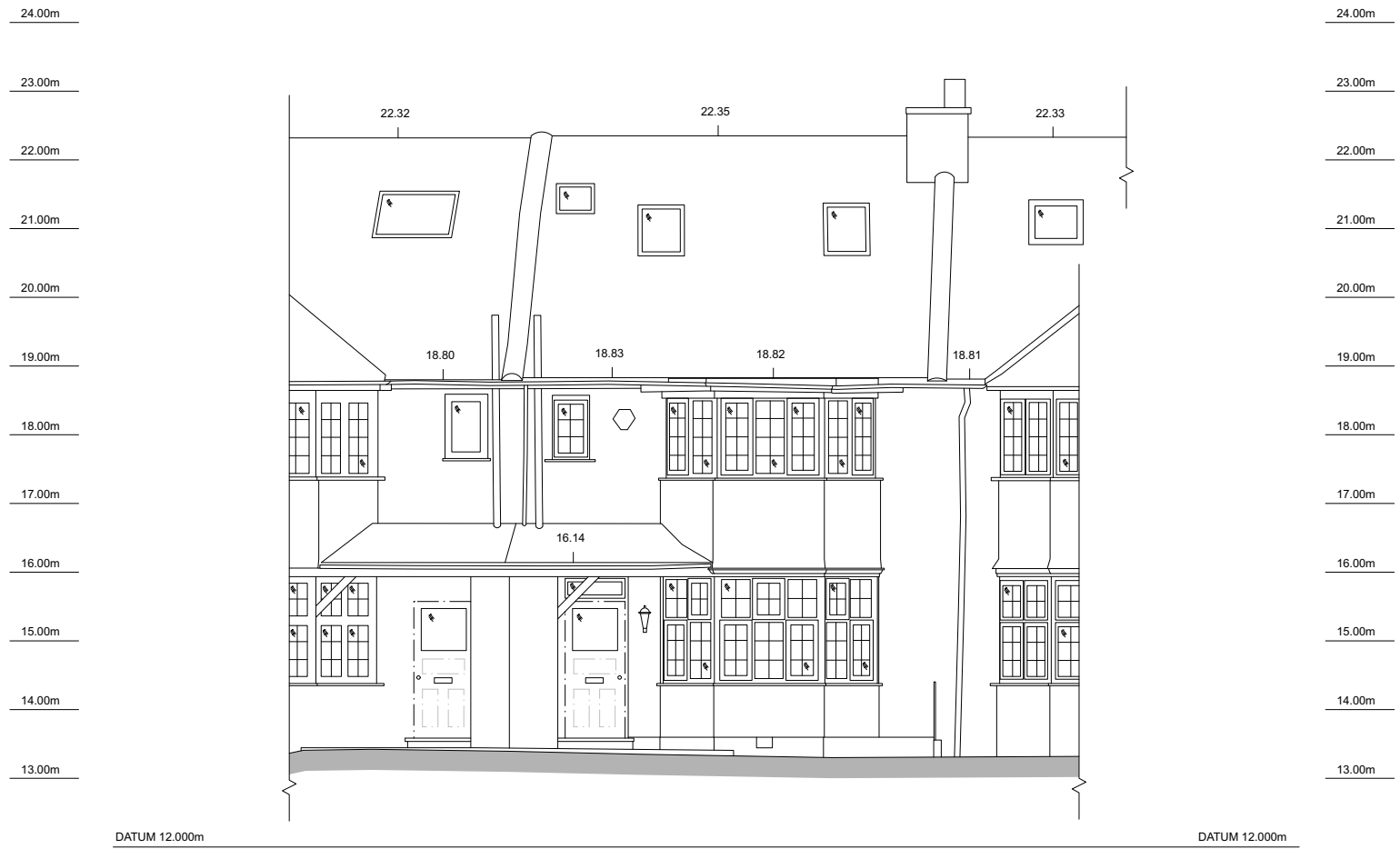
FRONT ELEVATION
