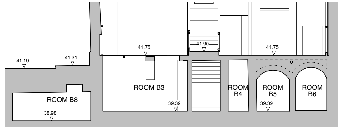
Section B-B : Basement Prior to Breach
