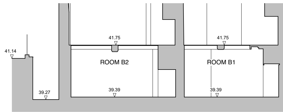
Section A-A : Basement Prior to Breach
