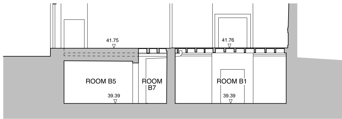
Section C-C : Basement Prior to Breach
