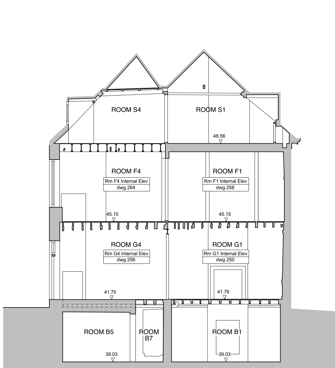
Section C-C : Existing
