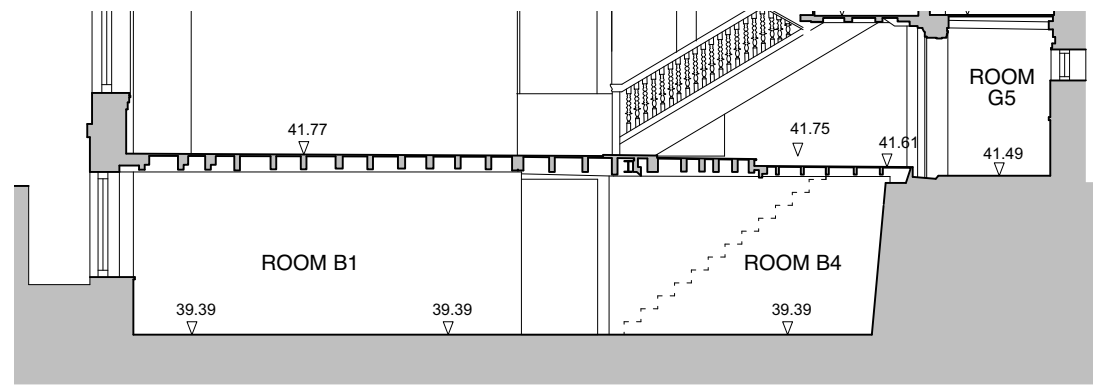
Section D-D : Basement Prior to Breach
