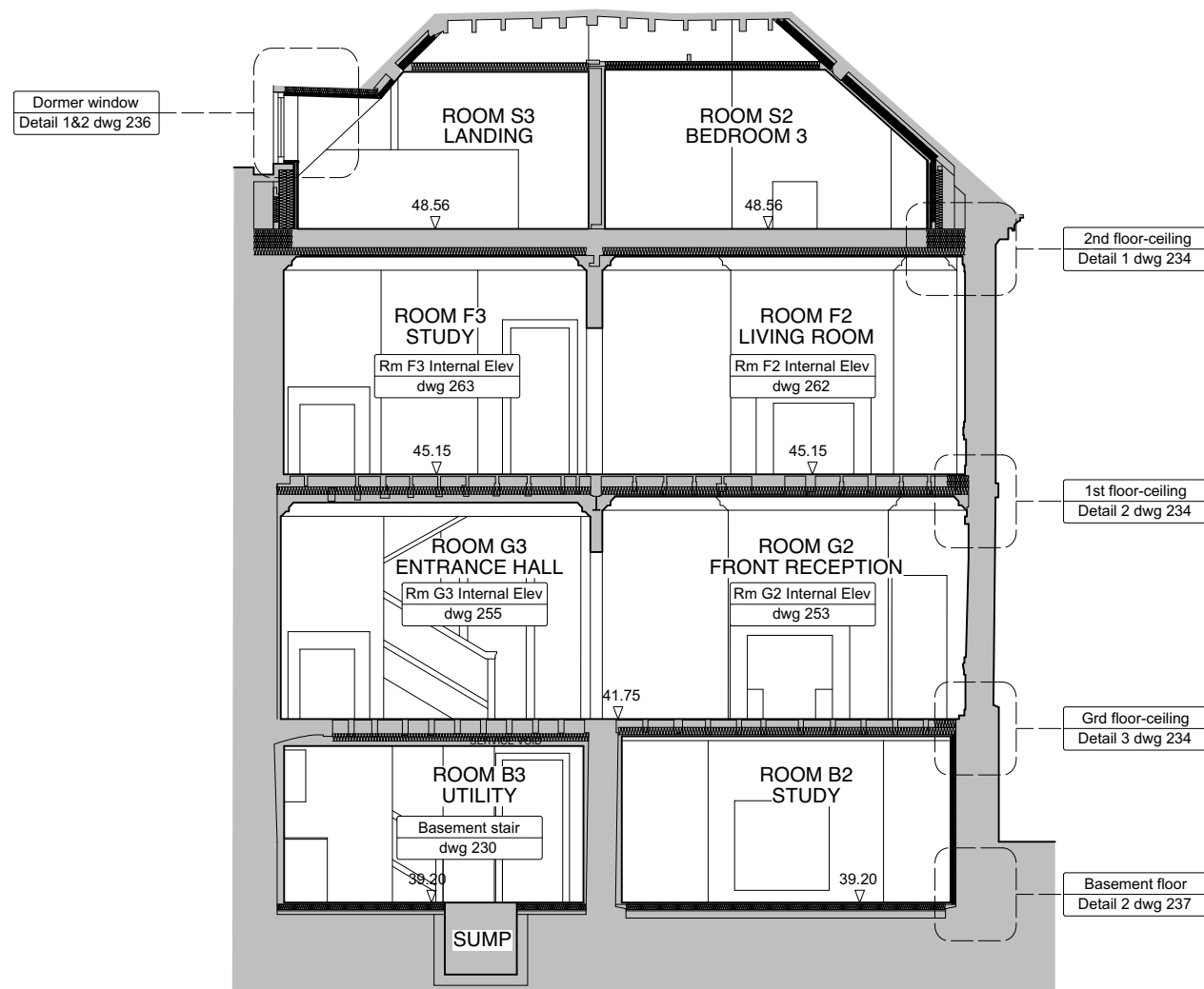
Section E-E : Proposed
