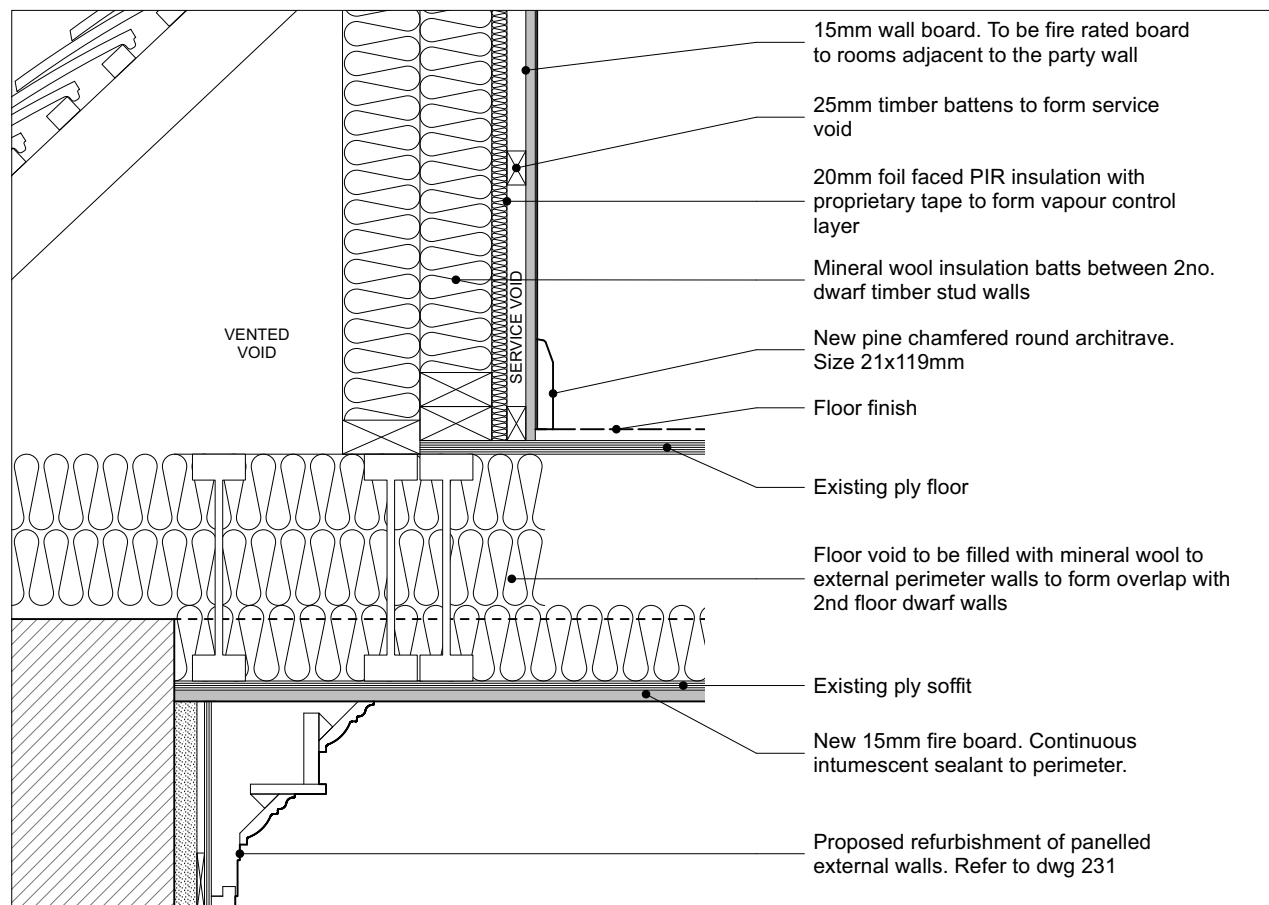
Detail 1: First to Second Floor External Wall Detail to Main Building 30 minute fire rating
