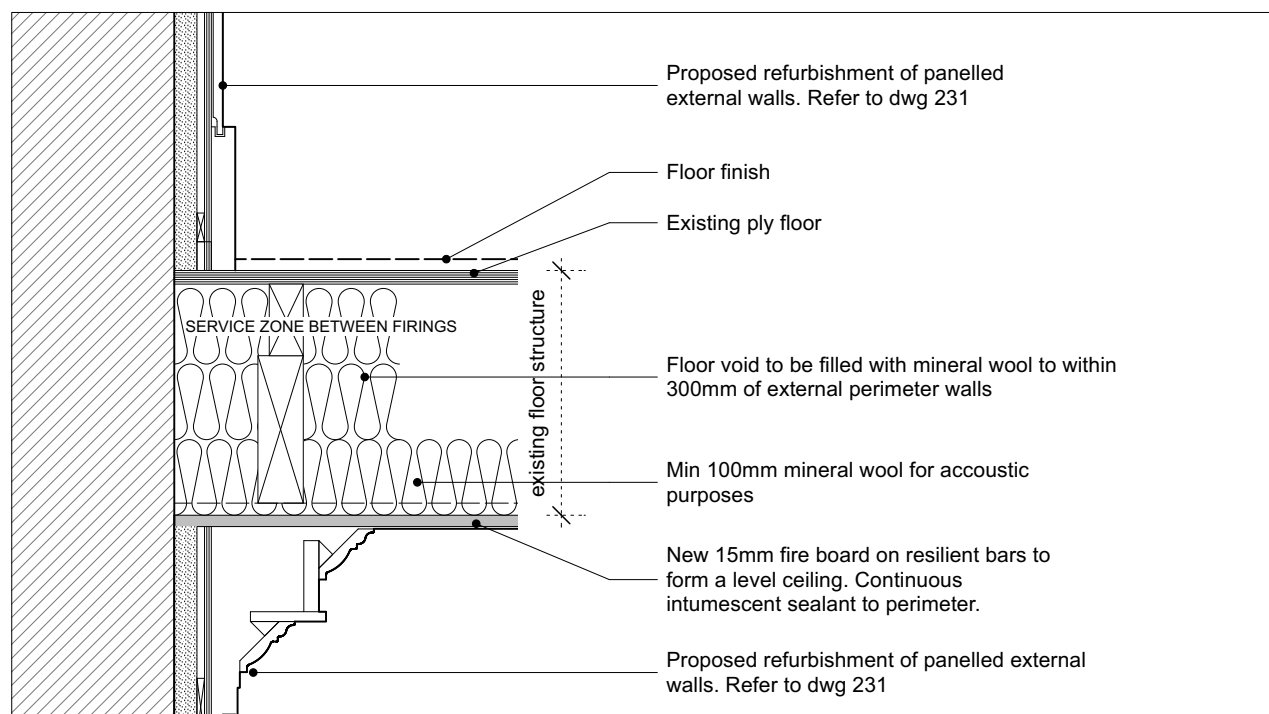
Detail 2: Ground to First Floor External Wall Detail to Main Building 30 minute fire rating
