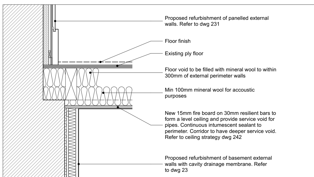
Detail 3: Basement to Ground Floor External Wall Detail to Main Building 60 minute fire rating
