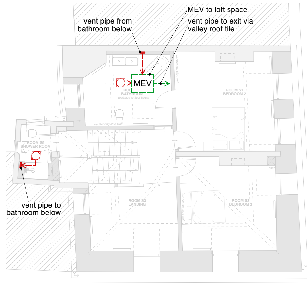
Second Floor Ventilation Strategy
