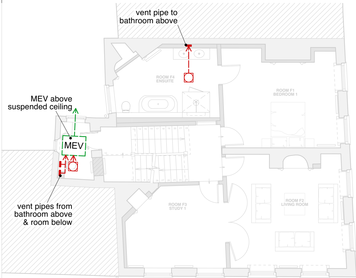
First Floor Ventilation Strategy
