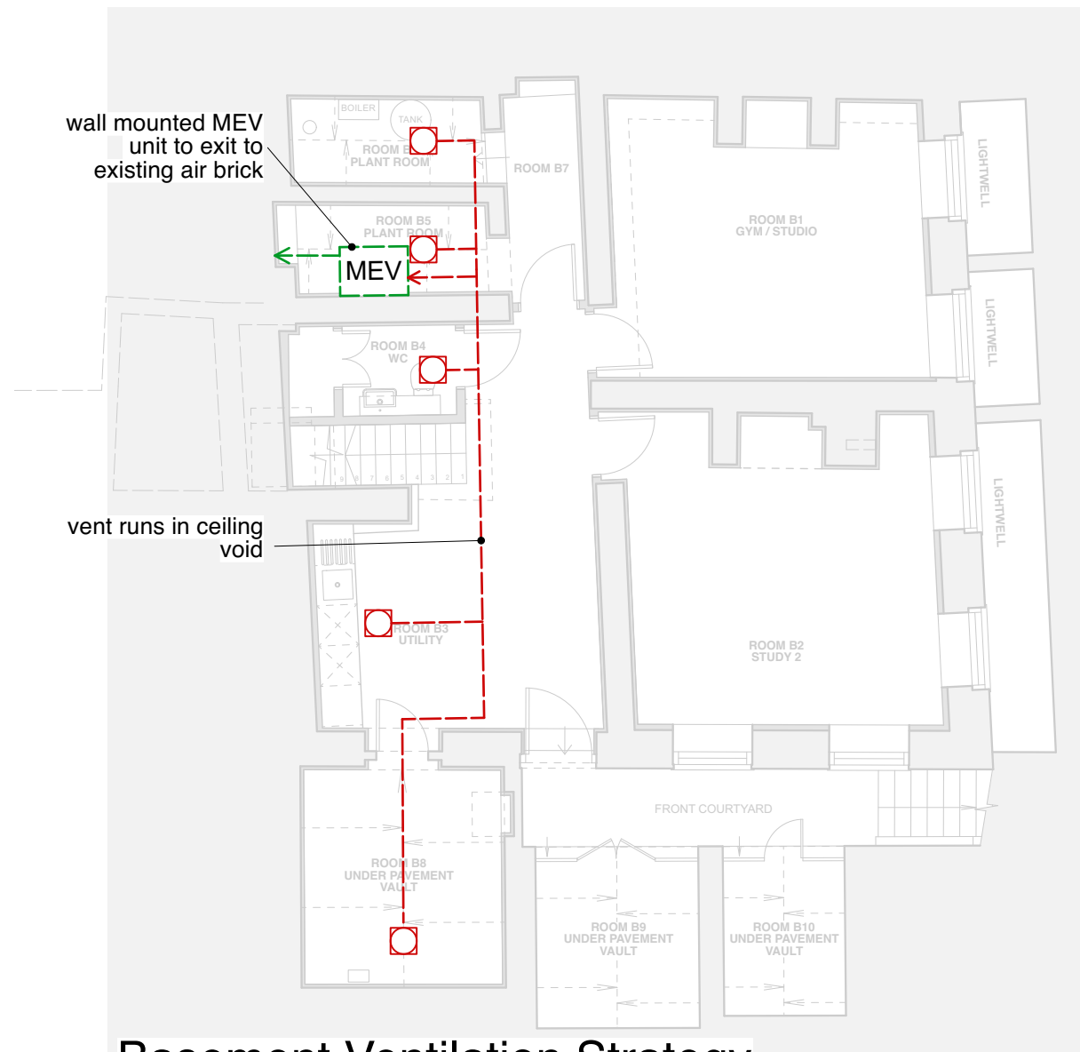
Basement Ventilation Strategy
