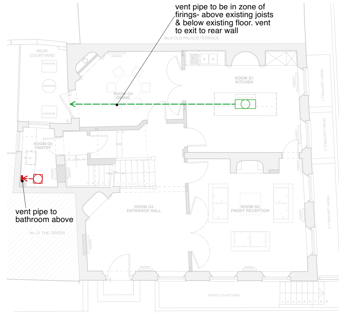
Ground Floor Ventilation Strategy
