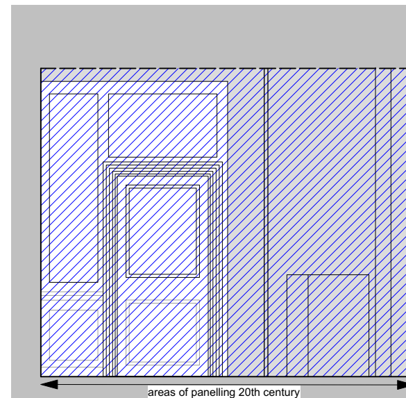
Elevation D
