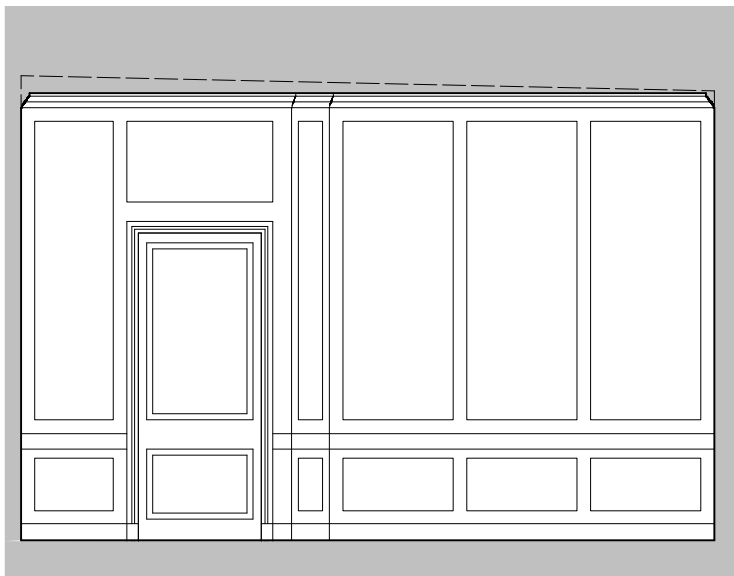
Elevation C
