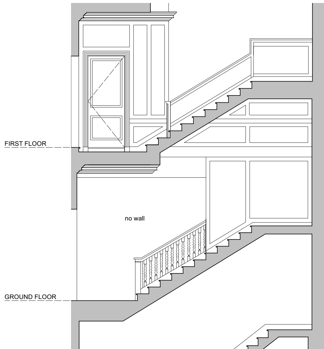
Elevation C
