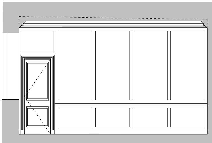
Elevation C
