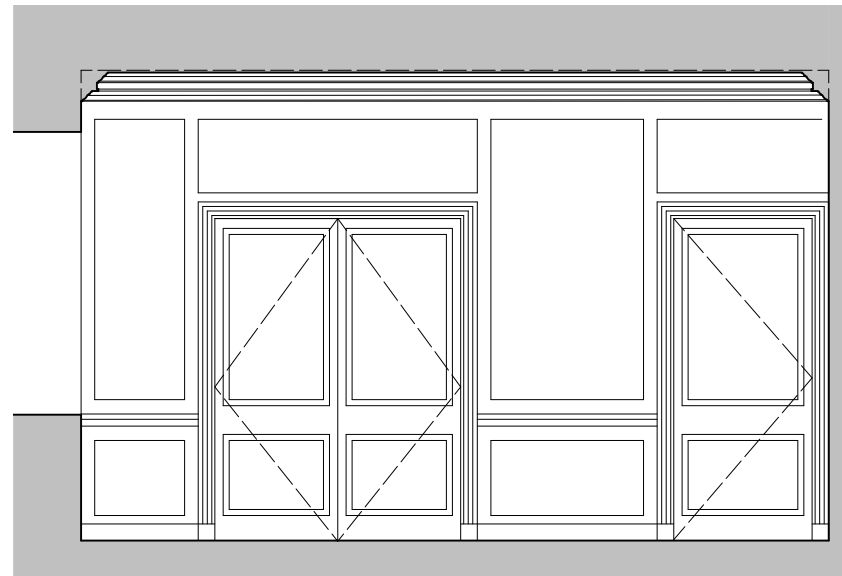
Elevation D
