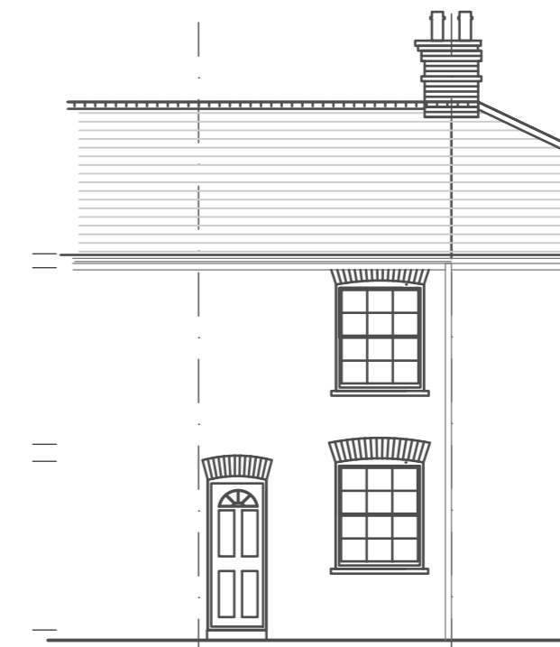
Front Elevation
