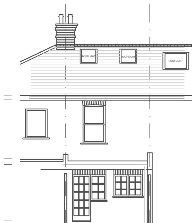
Rear Elevation
