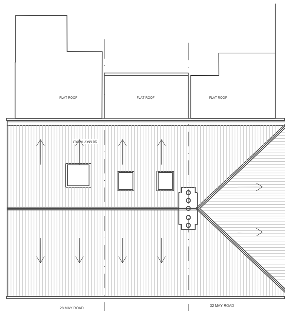
Roof Plan
