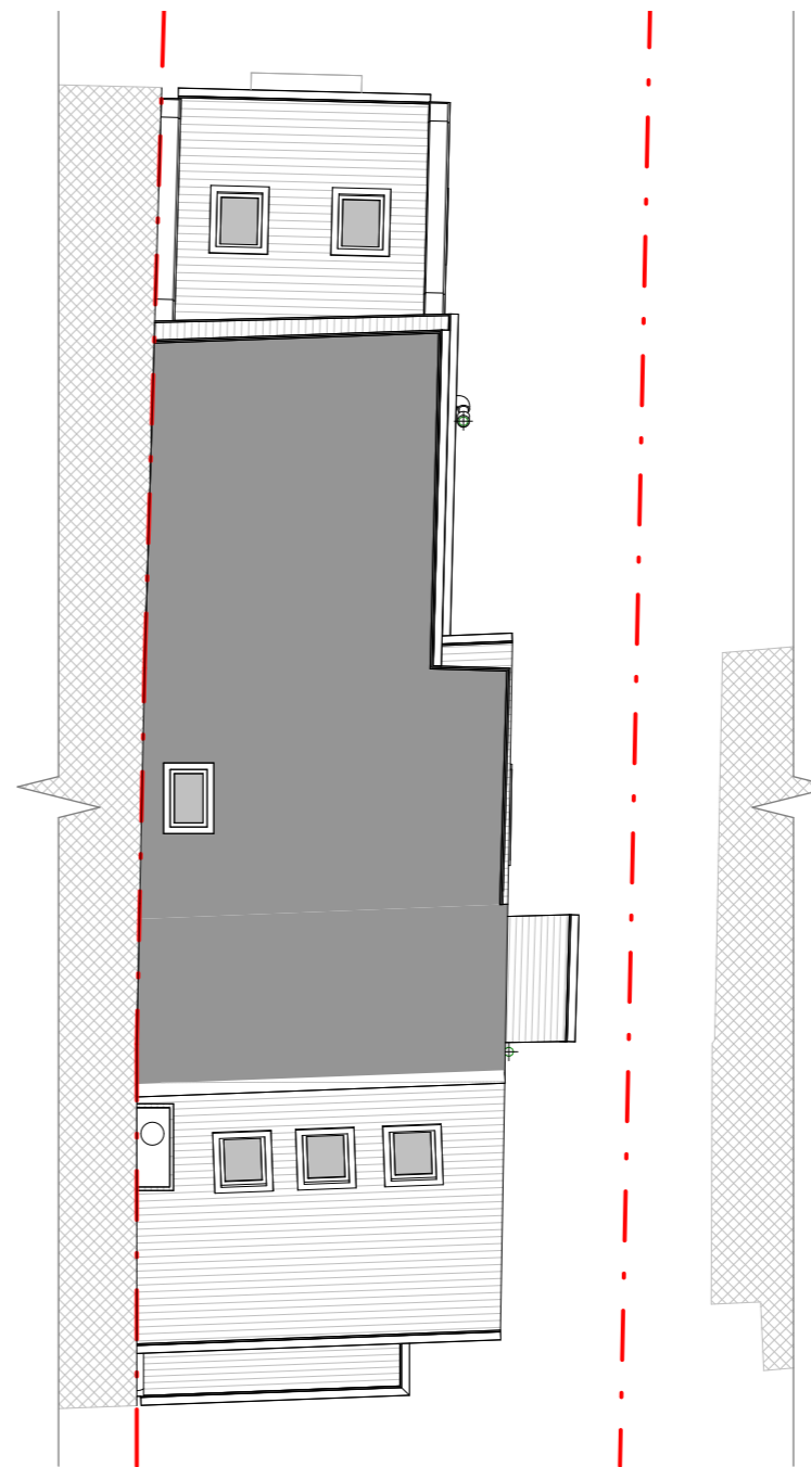
Roof Plan
