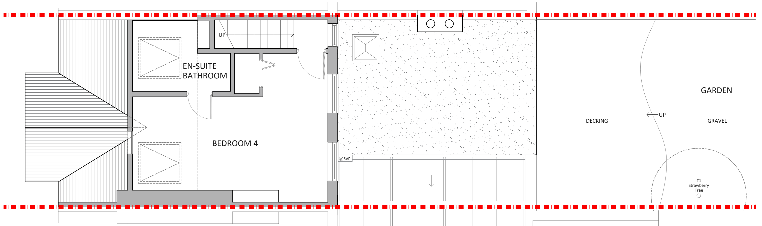
EXISTING LOFT FLOOR PLAN SCALE 1:50
