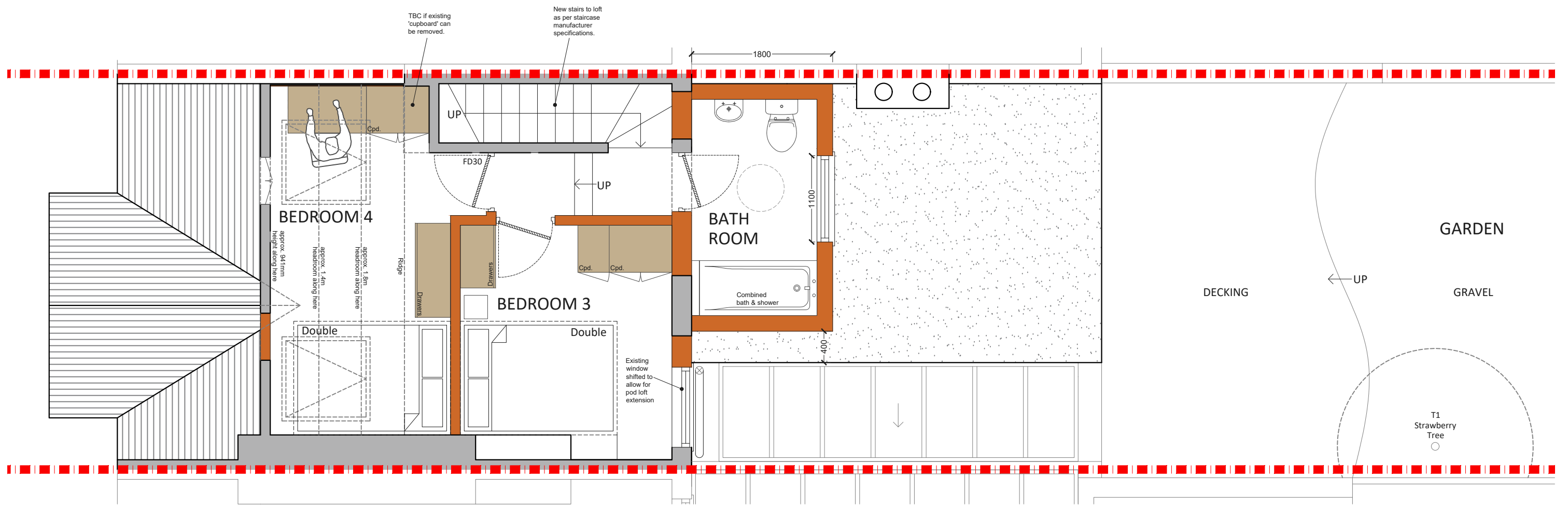
PROPOSED LOFT FLOOR PLAN SCALE 1:50
