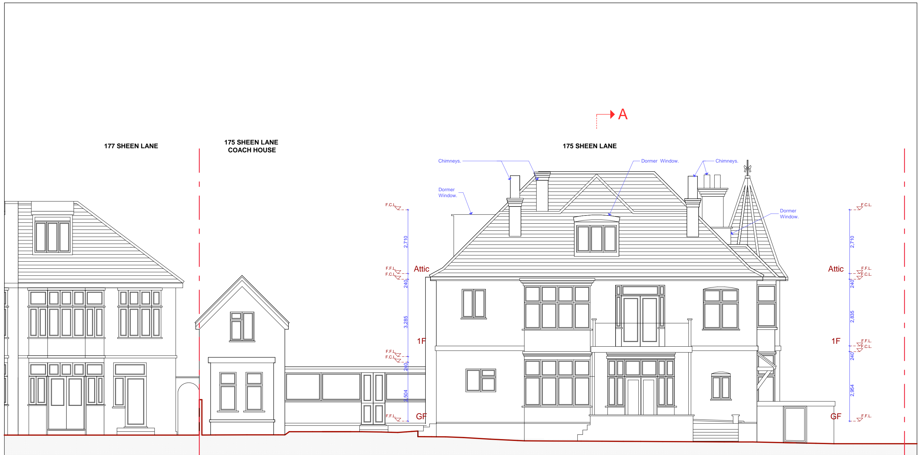
EXISTING EAST ELEVATION
