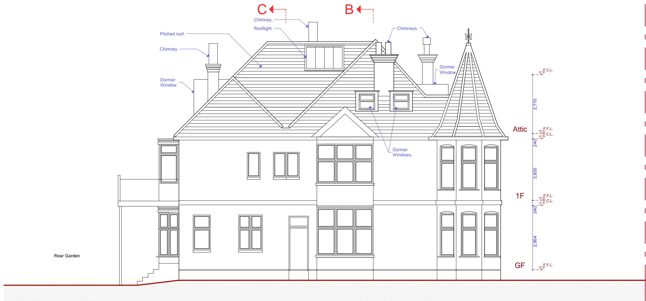
EXISTING NORTH ELEVATION
