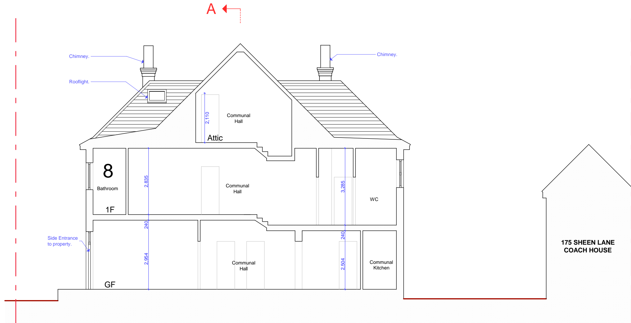
EXISTING SECTION C-C
