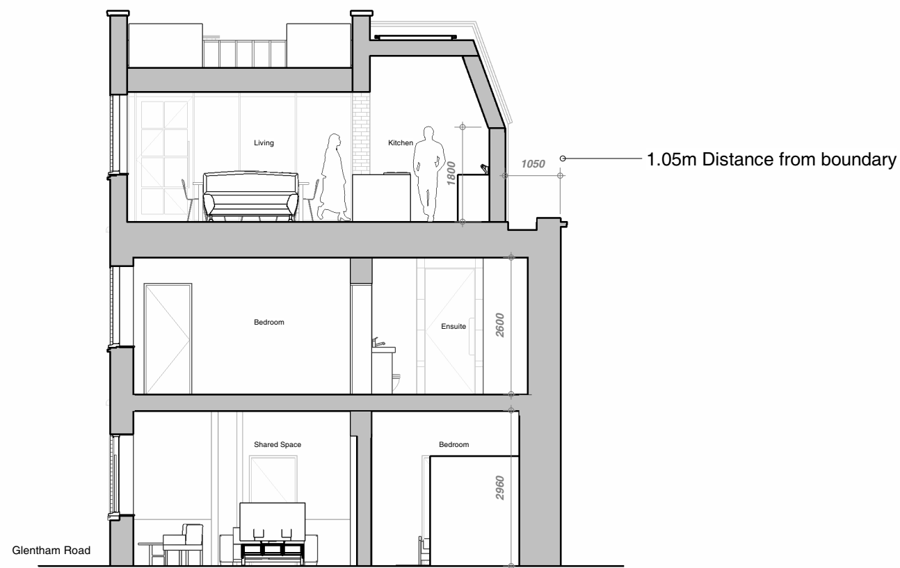
2 GA Proposed Section B-B 1 : 100
