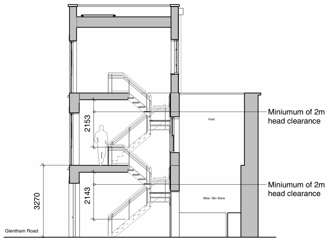
1 GA Proposed Section A-A 1 : 100
