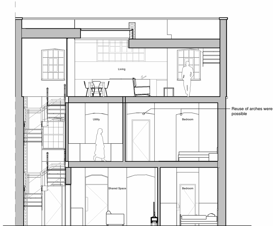
1 GA Proposed Section C-C 1 : 100
