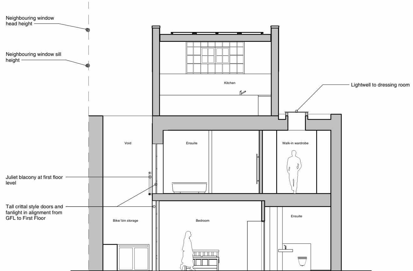
2 GA Proposed Section D-D 1 : 100
