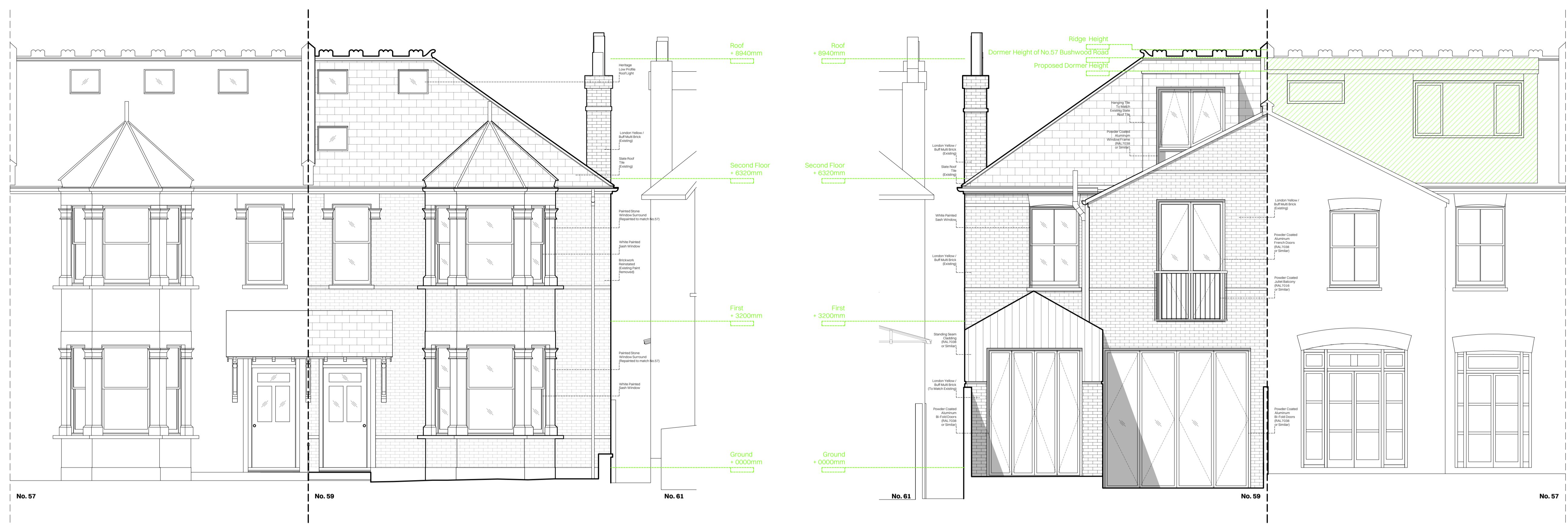
Proposed Front Elevation 1:50
