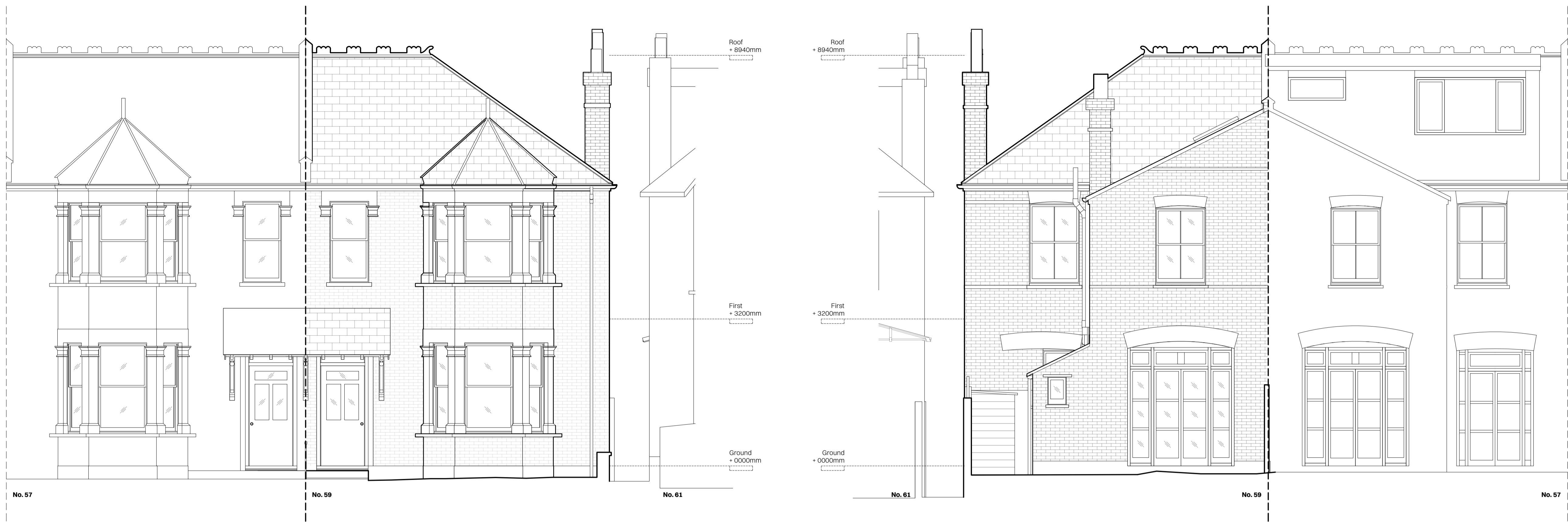
Existing Front Elevation 1:50
