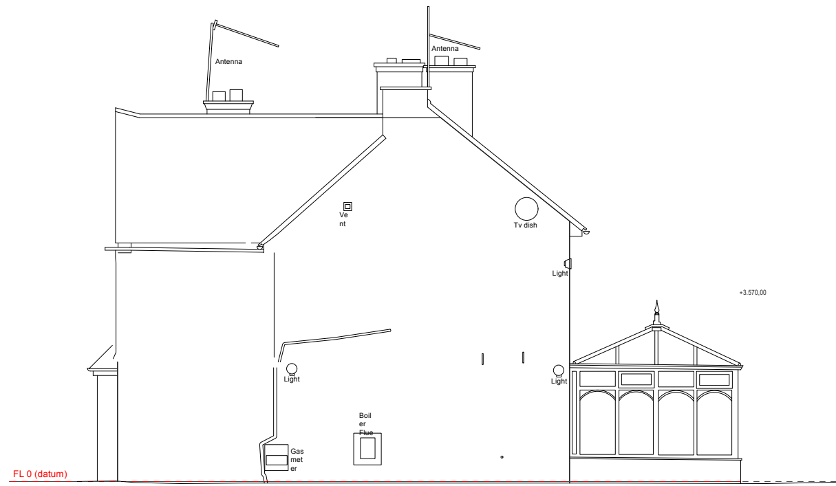
FRONT ELEVATION- WEST
