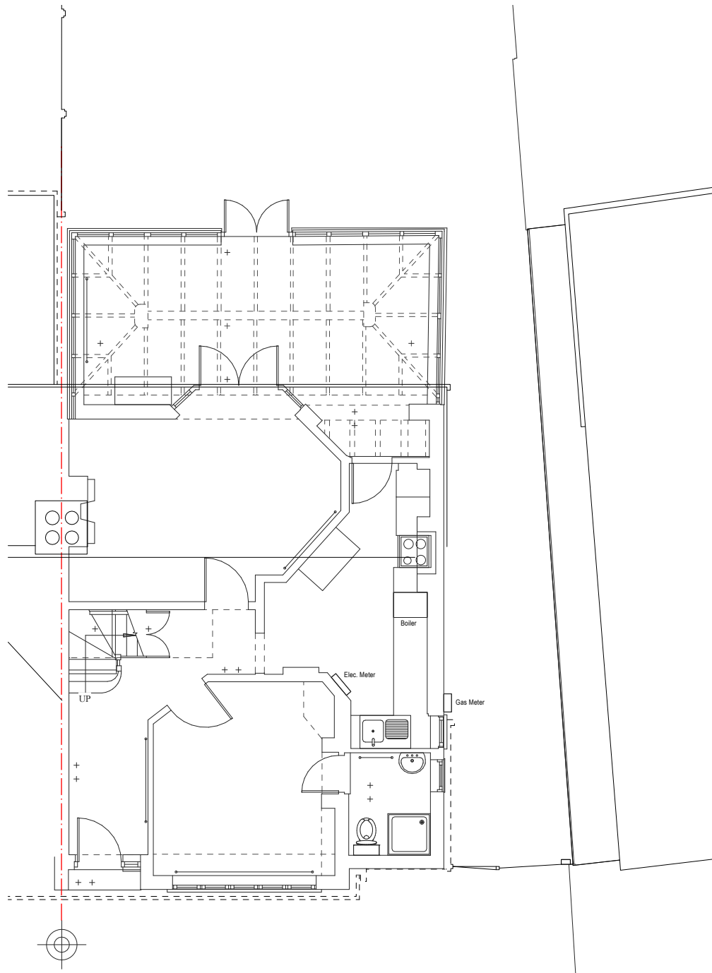
GROUND FLOOR
