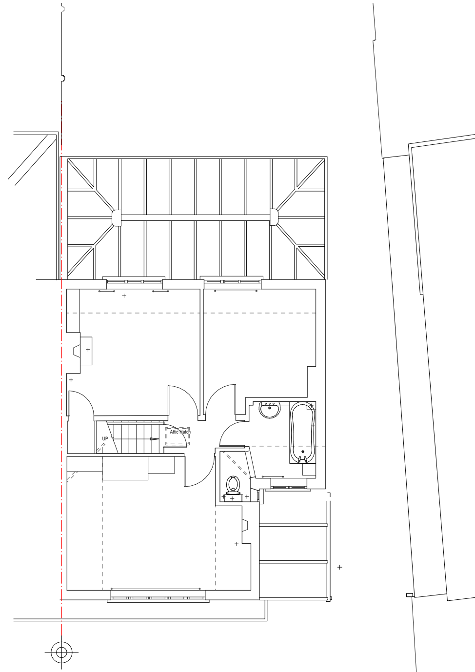
FIRST FLOOR
