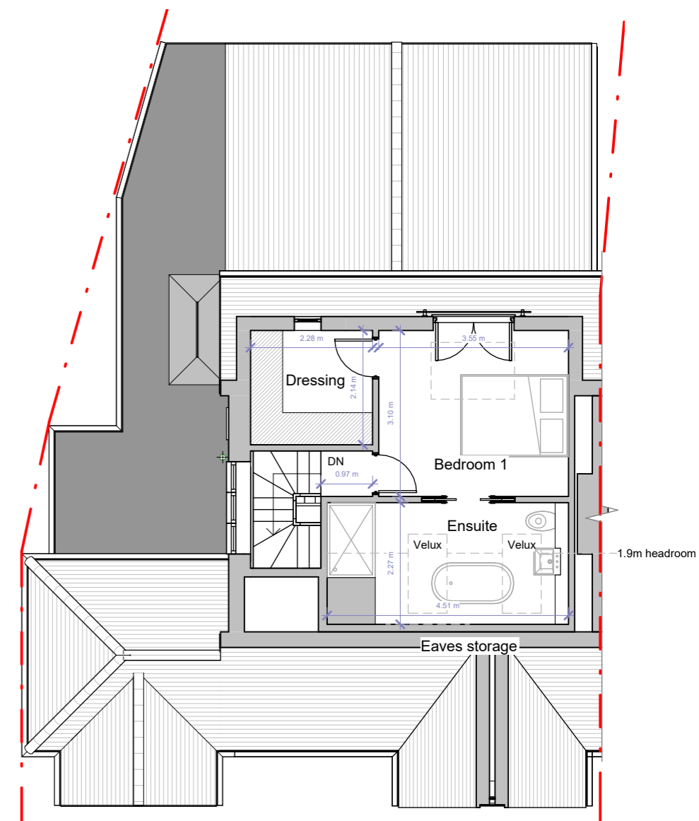
Second Floor
