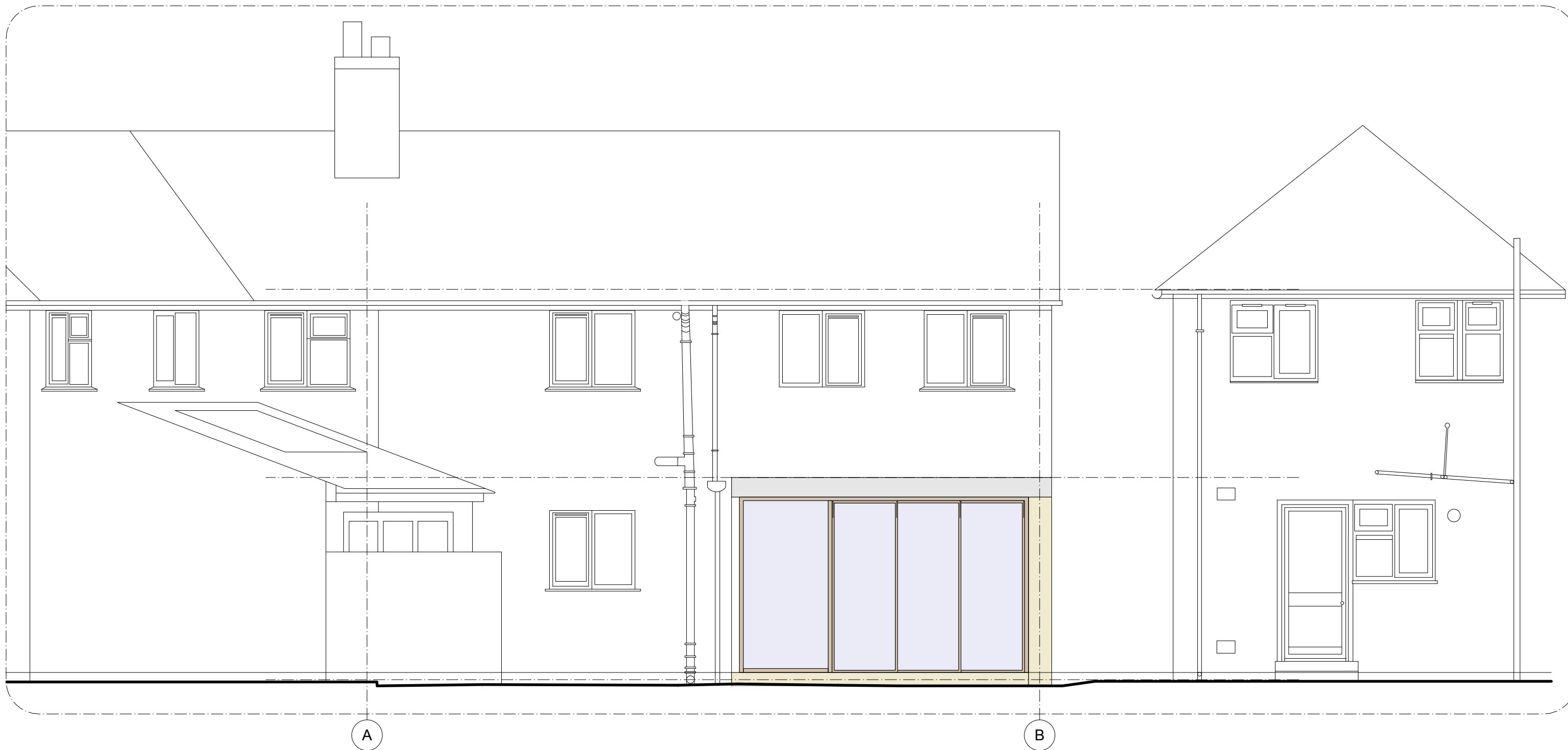
Rear Elevation
