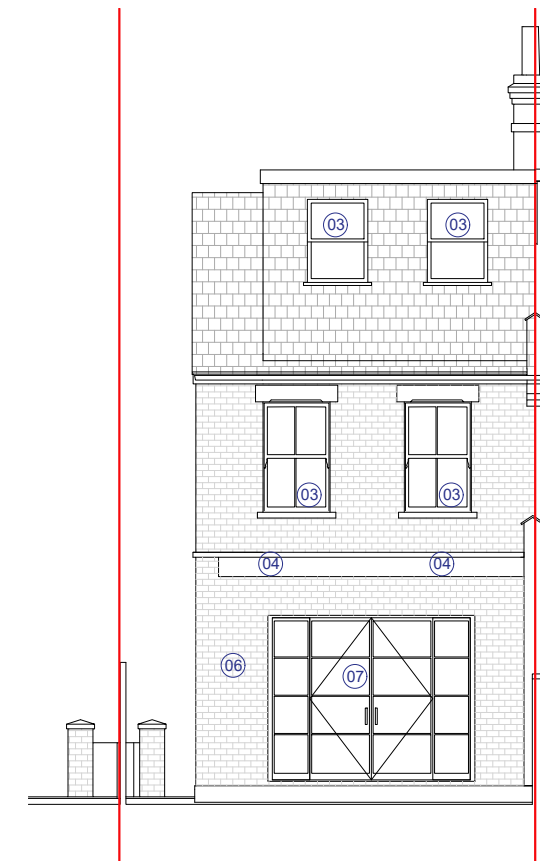
A3 1:100 PROPOSED REAR ELEVATION
