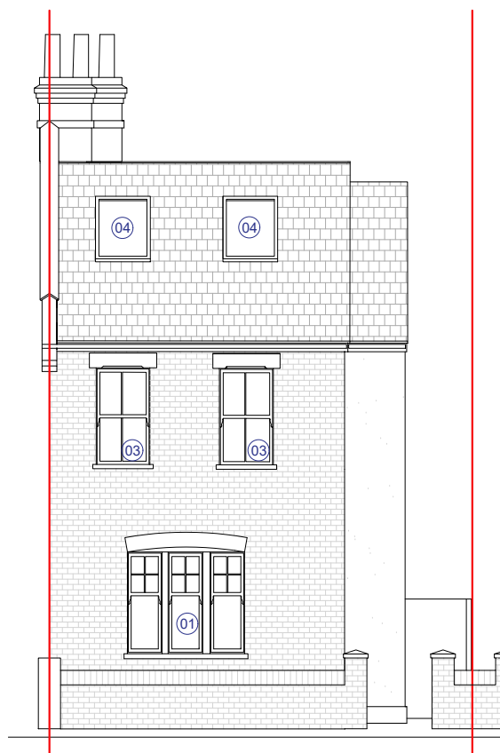
A3 PROPOSED FRONT ELEVATION 1:100
