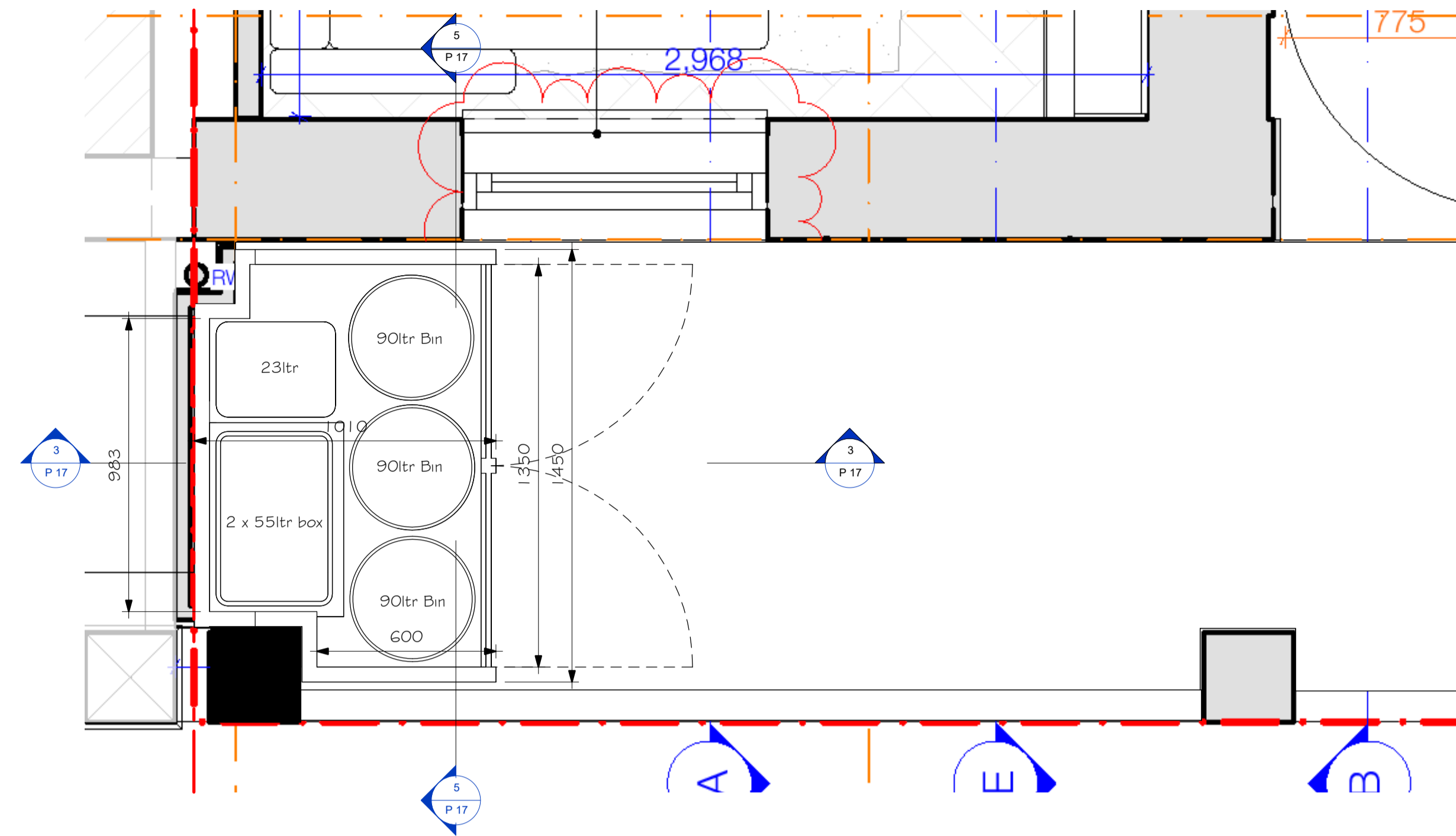
1 Refuse and Recycling Storage Plan 1 : 15
