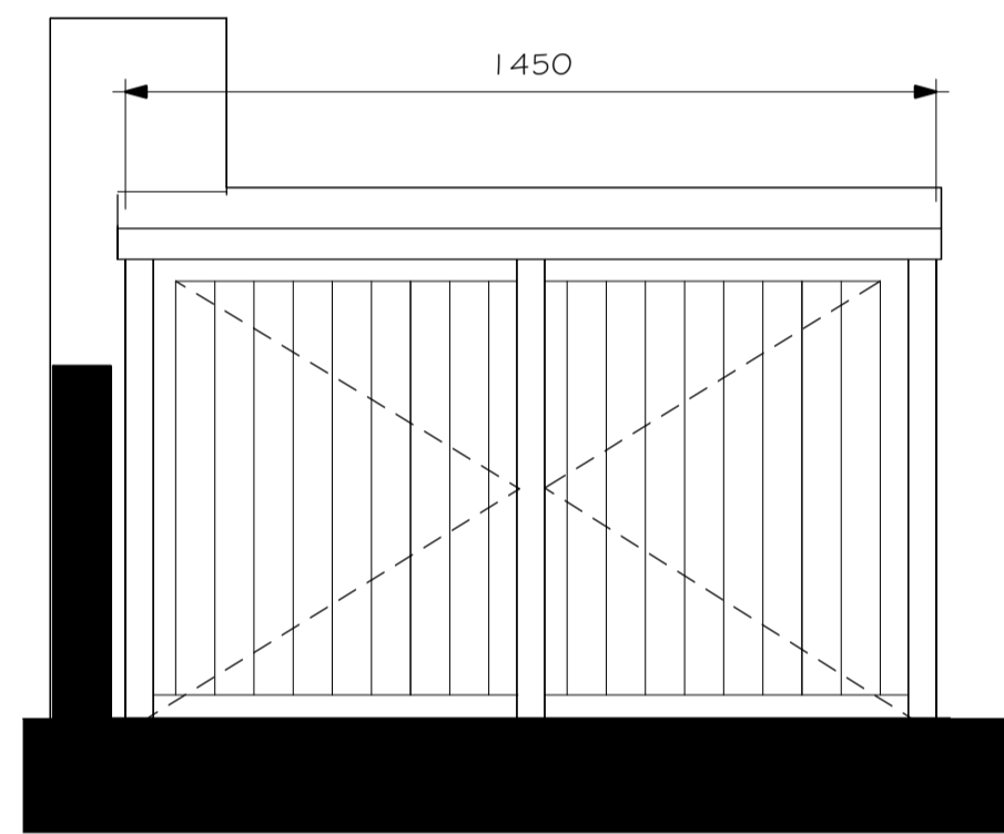
2 Bin Store Front Elevation 1 : 15
