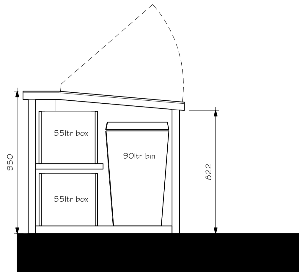
3 Bin Store Section 1 1 : 15
