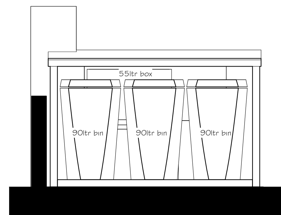
5 Bin Store Section 2 1 : 15
