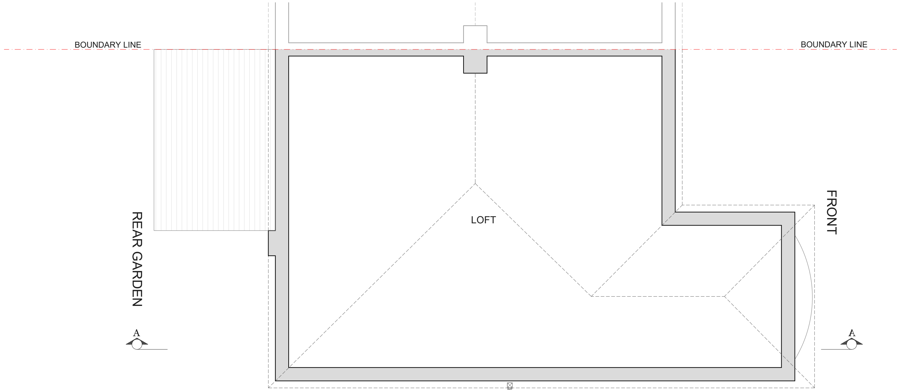
EXISTING LOFT FLOOR PLAN SCALE 1:50
