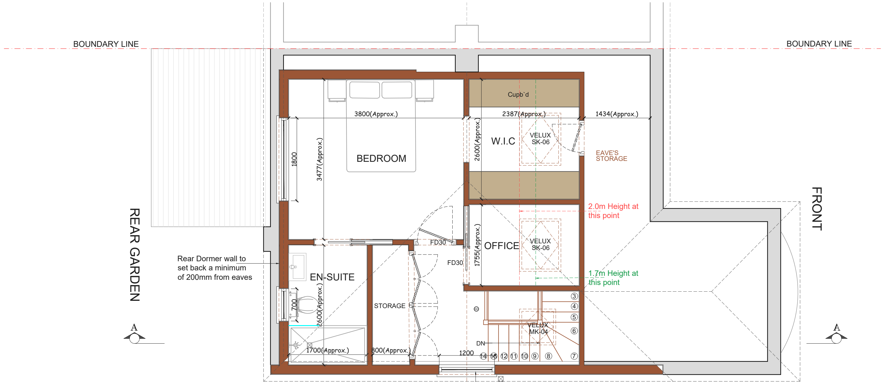
PROPOSED LOFT FLOOR PLAN SCALE 1:50
