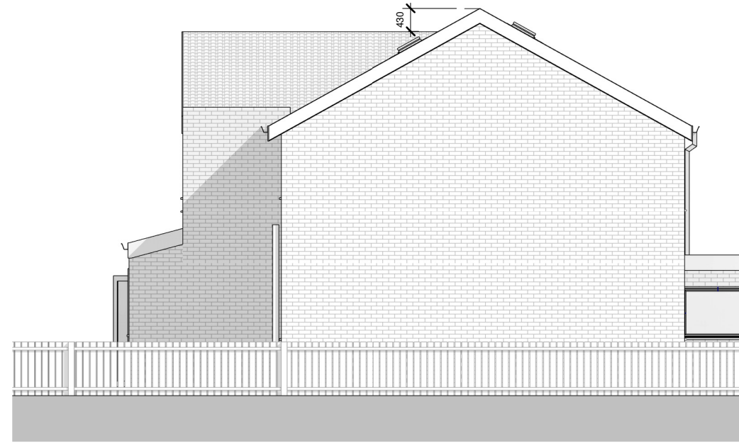
Left elevation
