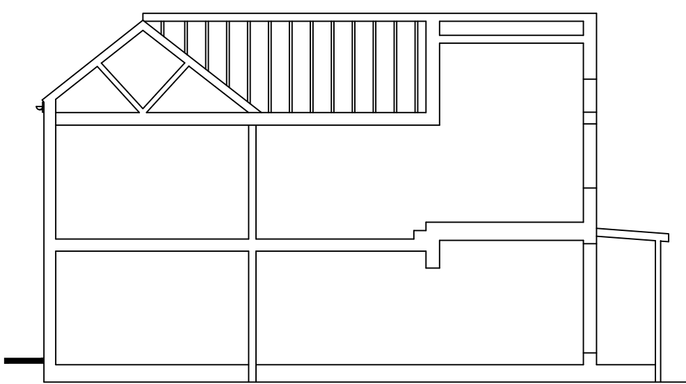
Existing Section A - A 1:100
