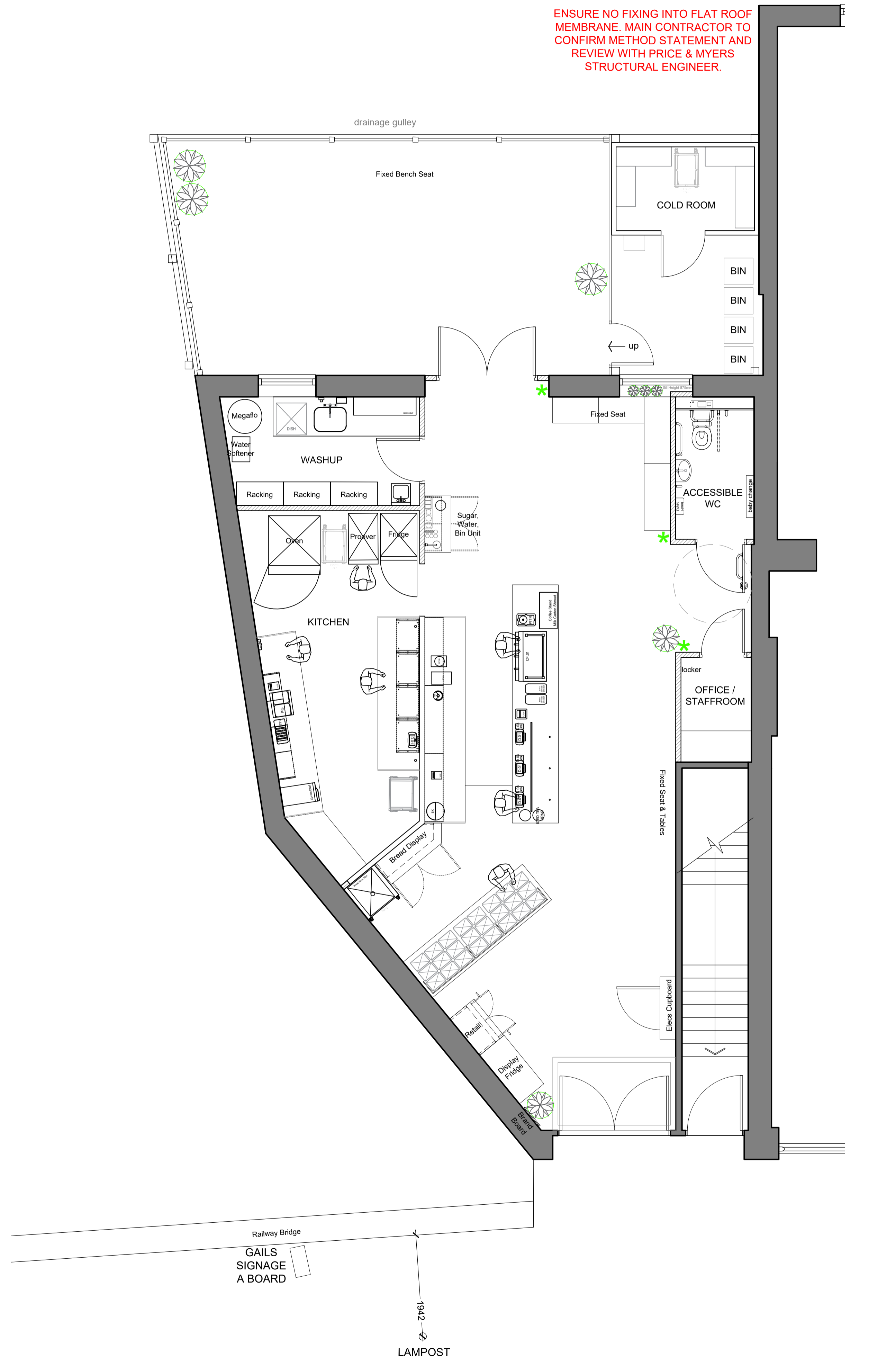
Proposed Plan 1:50
