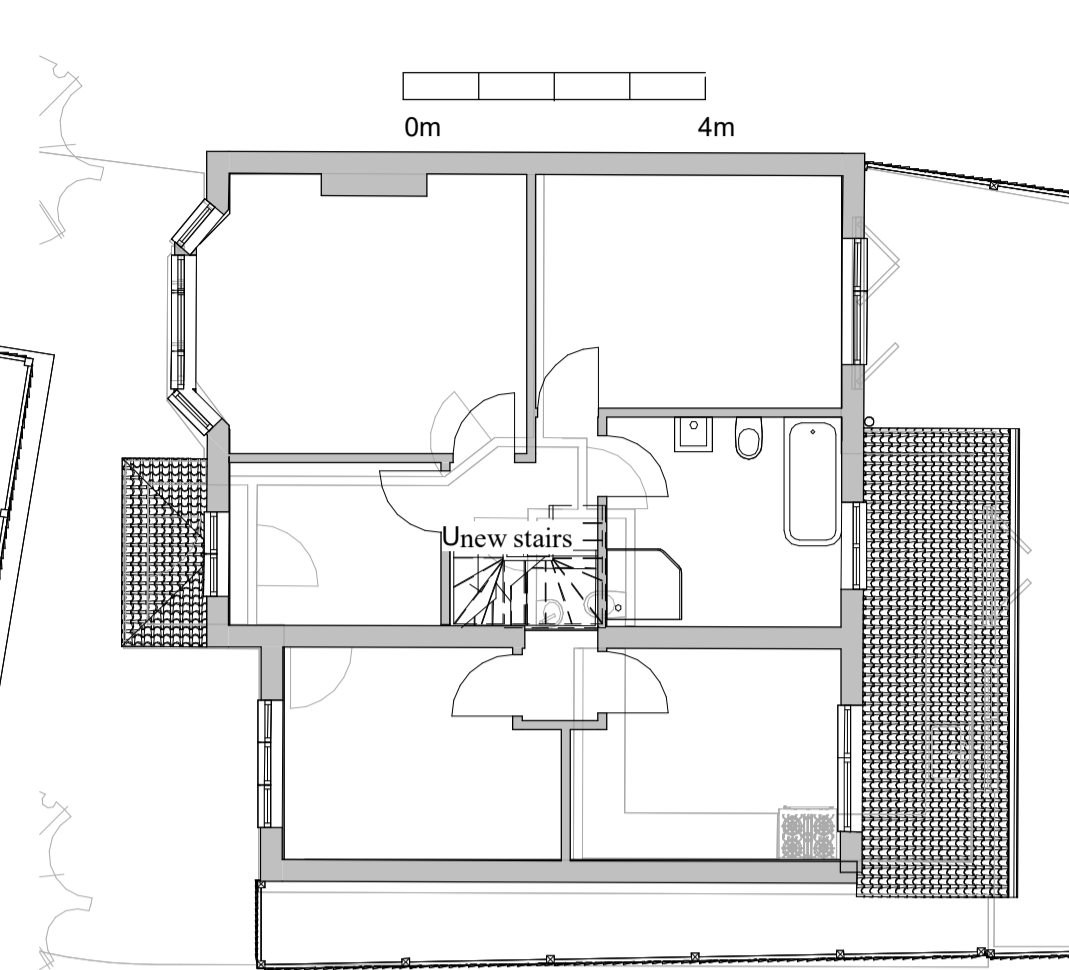
First Flr - proposed 1 : 100
