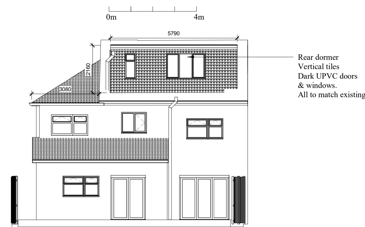
Rear Elev - proposed 1 : 100
