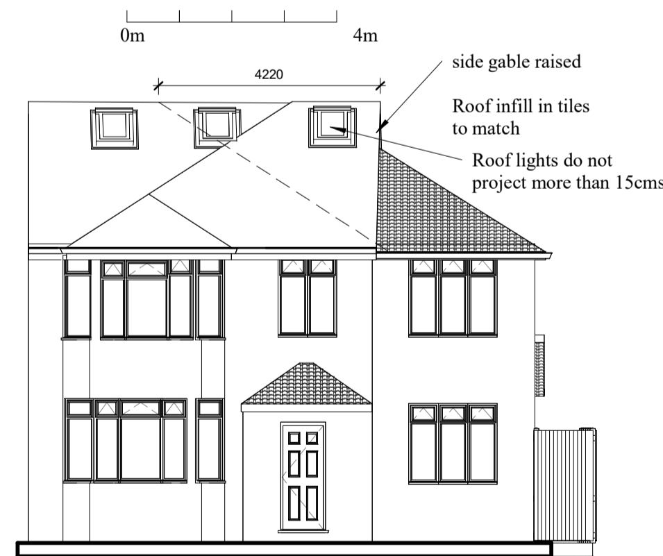
Front elev - proposed 1 : 100
