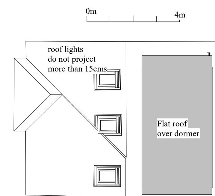
Roof - Proposed 1 : 100
