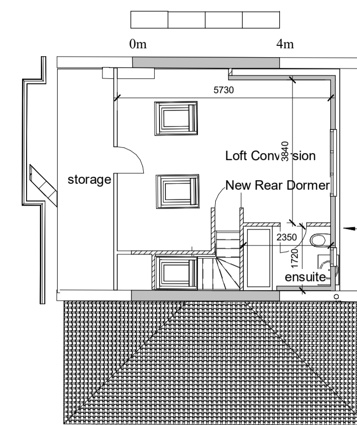
Second Flr - Proposed 1 : 100
