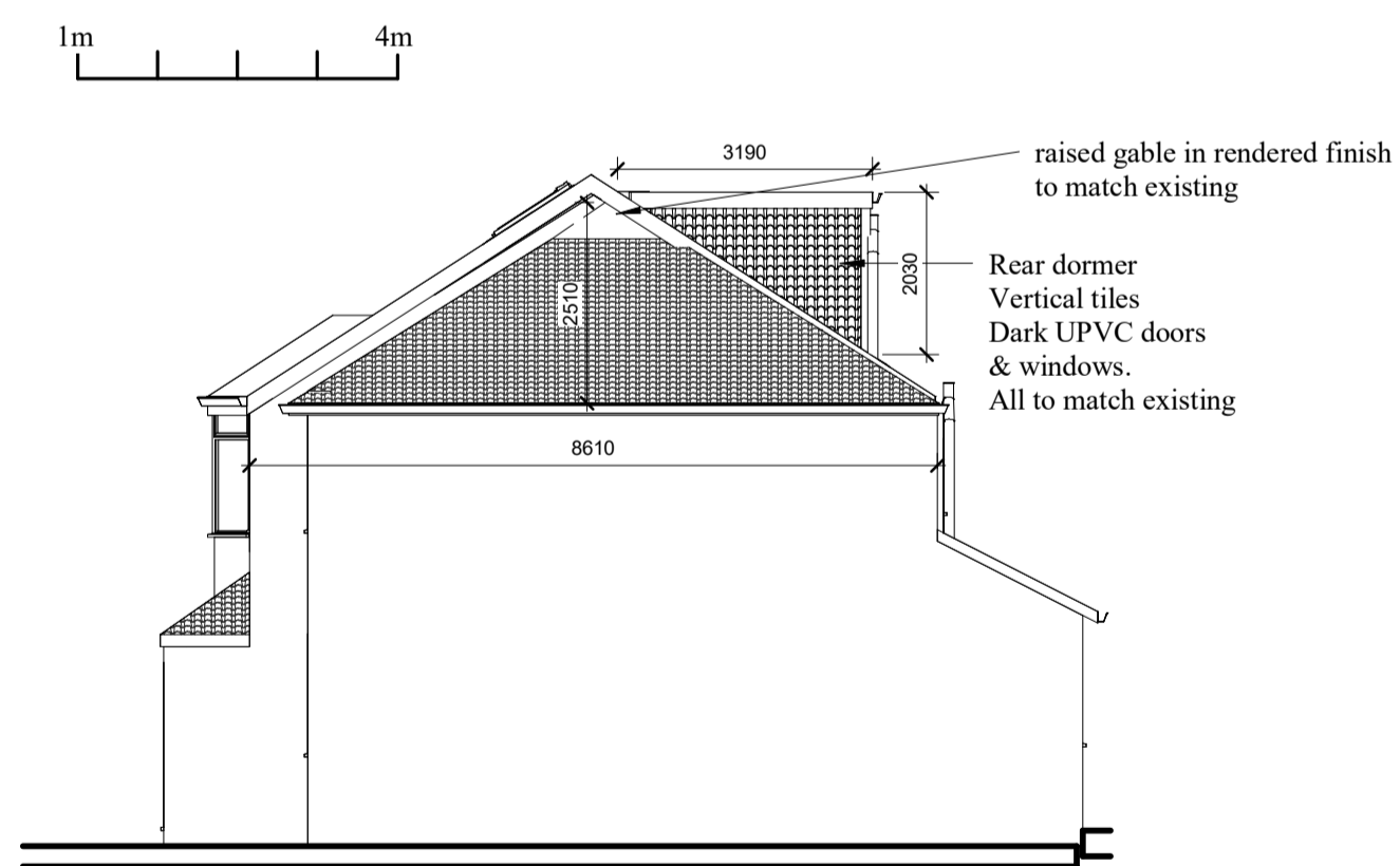
Side Elev - proposed 1 : 100
