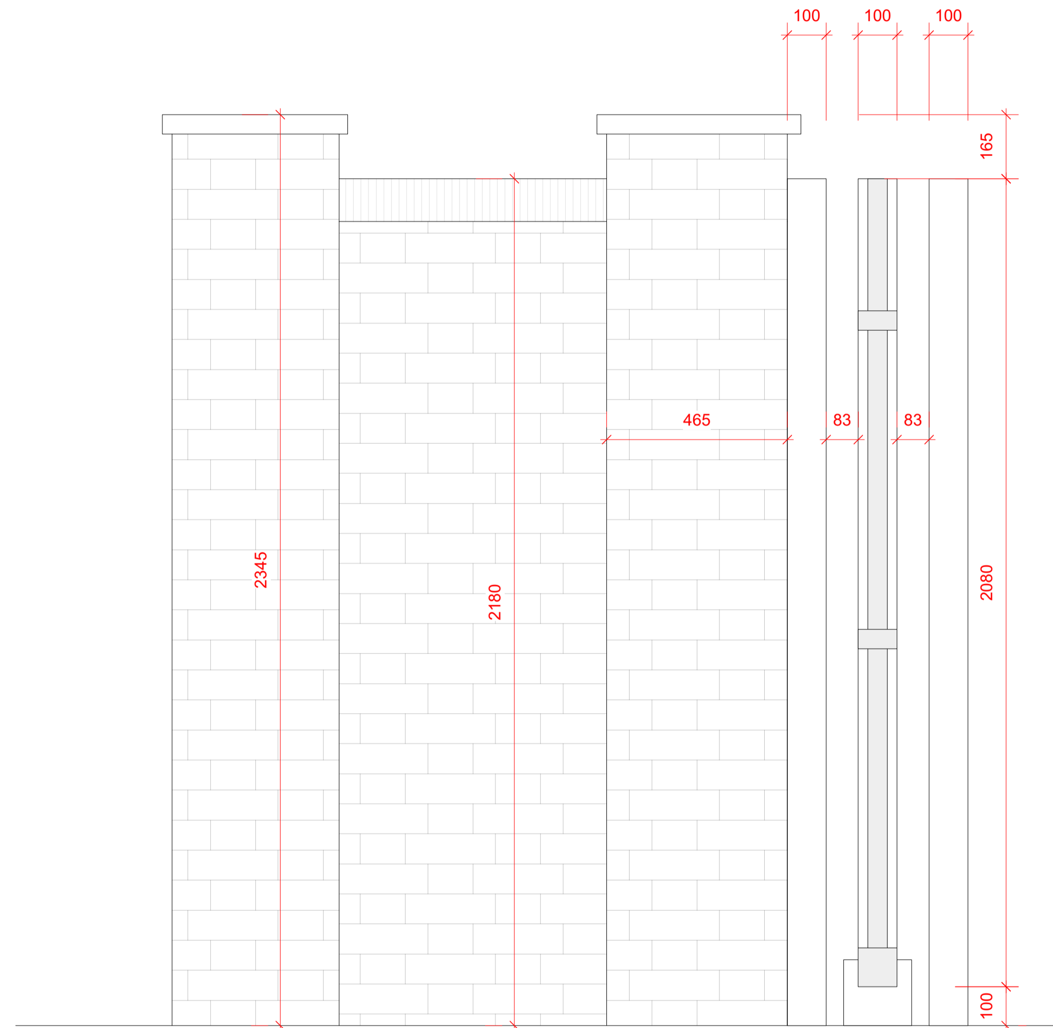
A Proposed Gate Section Scale 1:10
