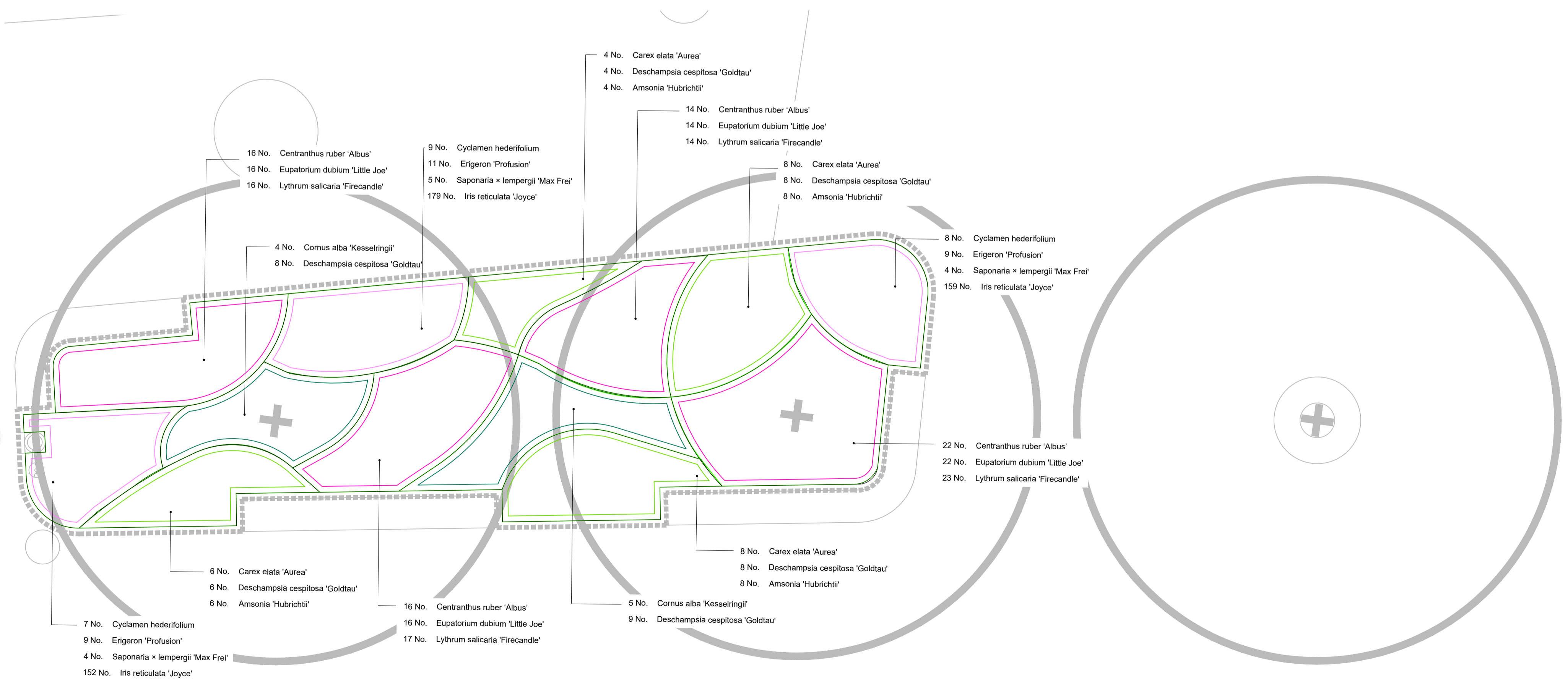
02 TYPICAL PLANTING PLAN - RIVERSIDE PLANTERS PLAN SCALE 1:50 @ A1
