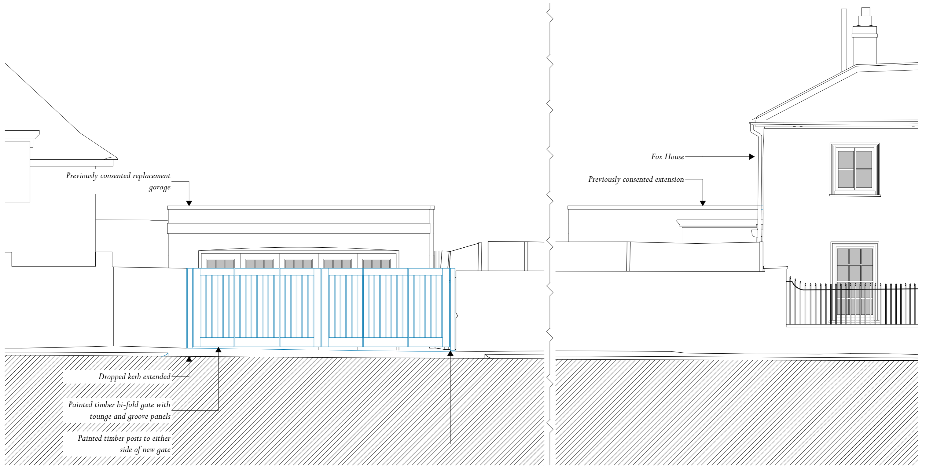
Gate Elevation - Proposed
