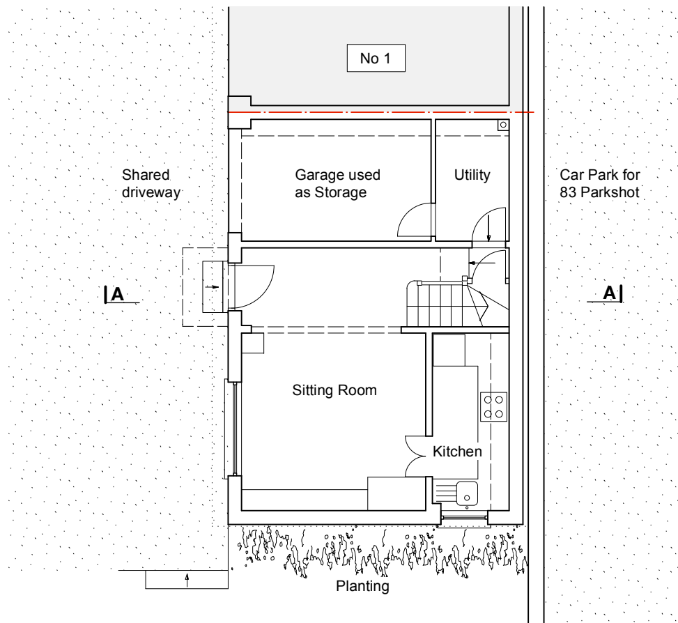
Ground Floor
