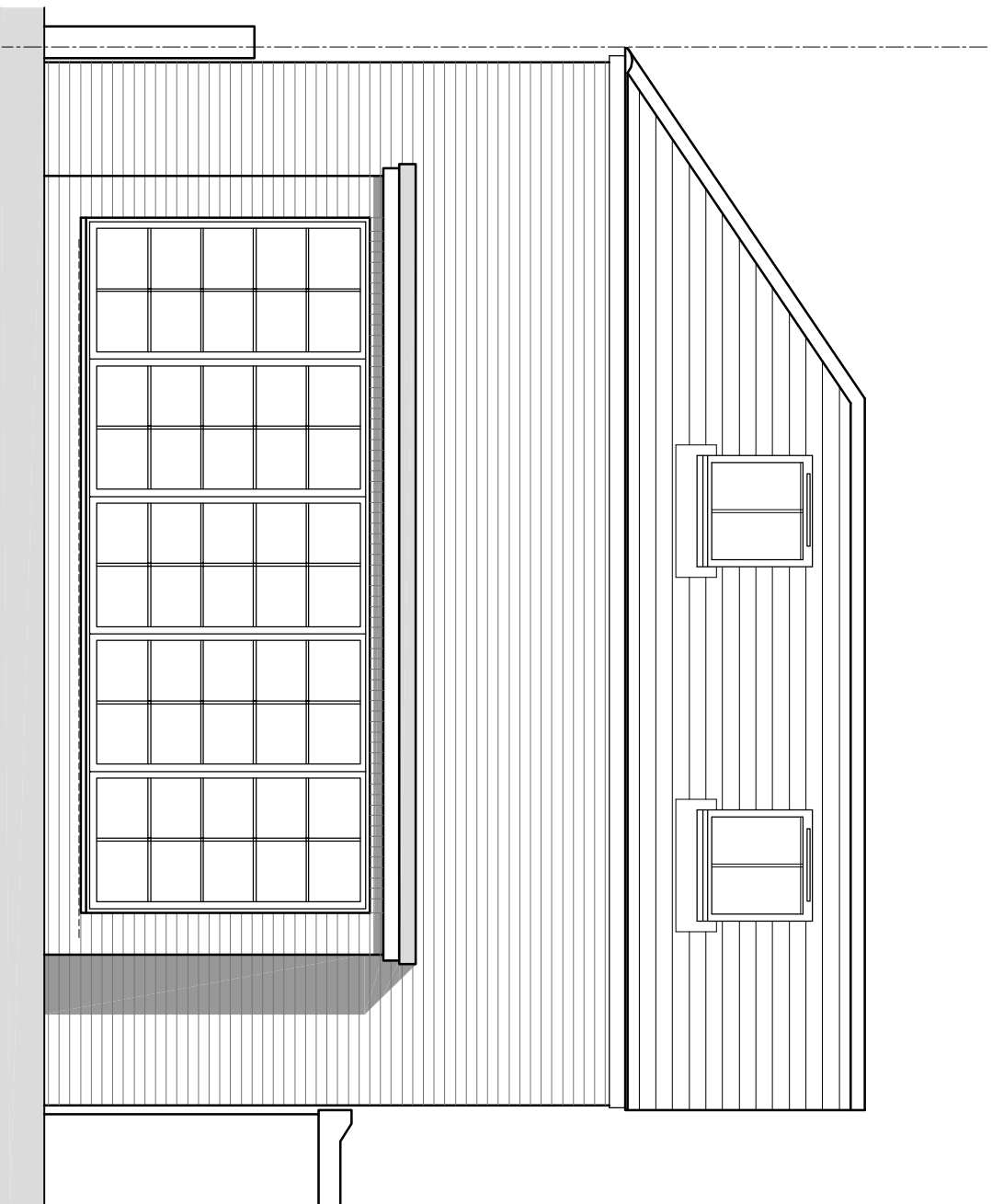
Proposed North East Facing Elevation
