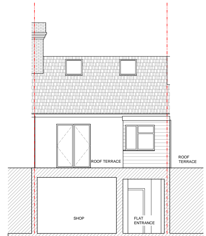
Section B
