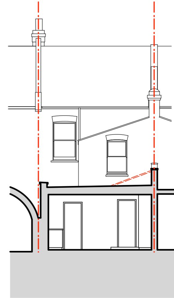
02 Proposed Section B-B
