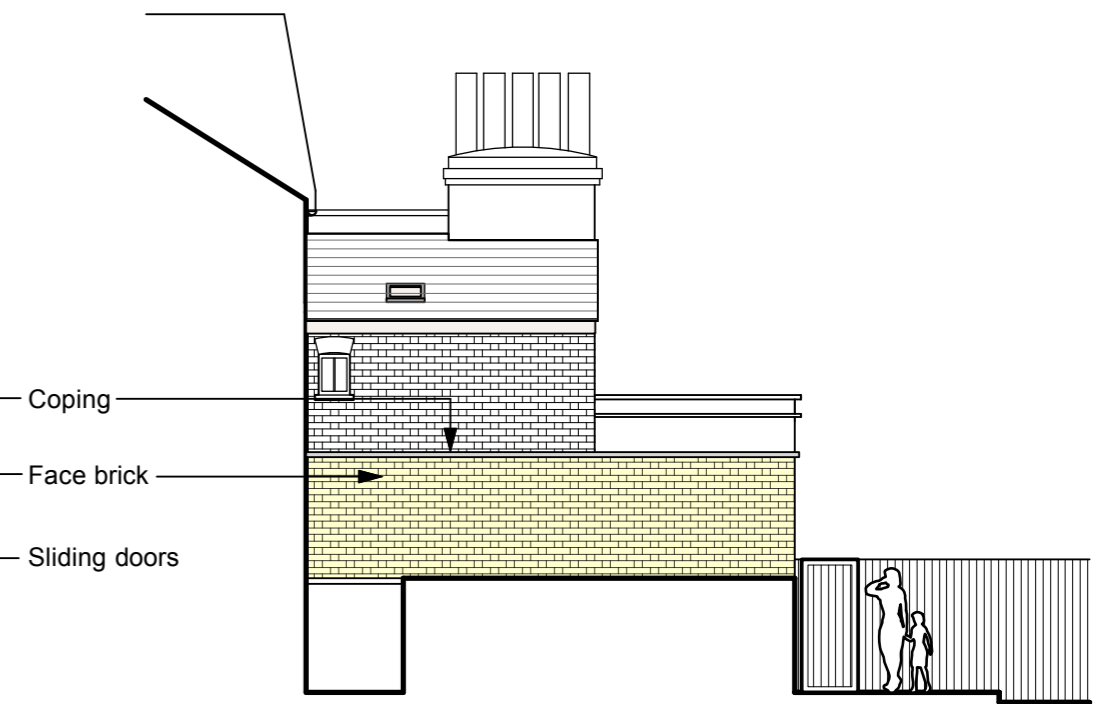
03 Proposed Side Elevation
