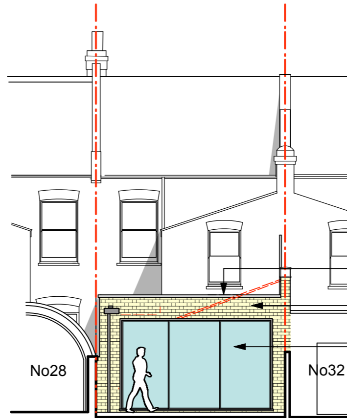
02 Proposed Rear Elevation
