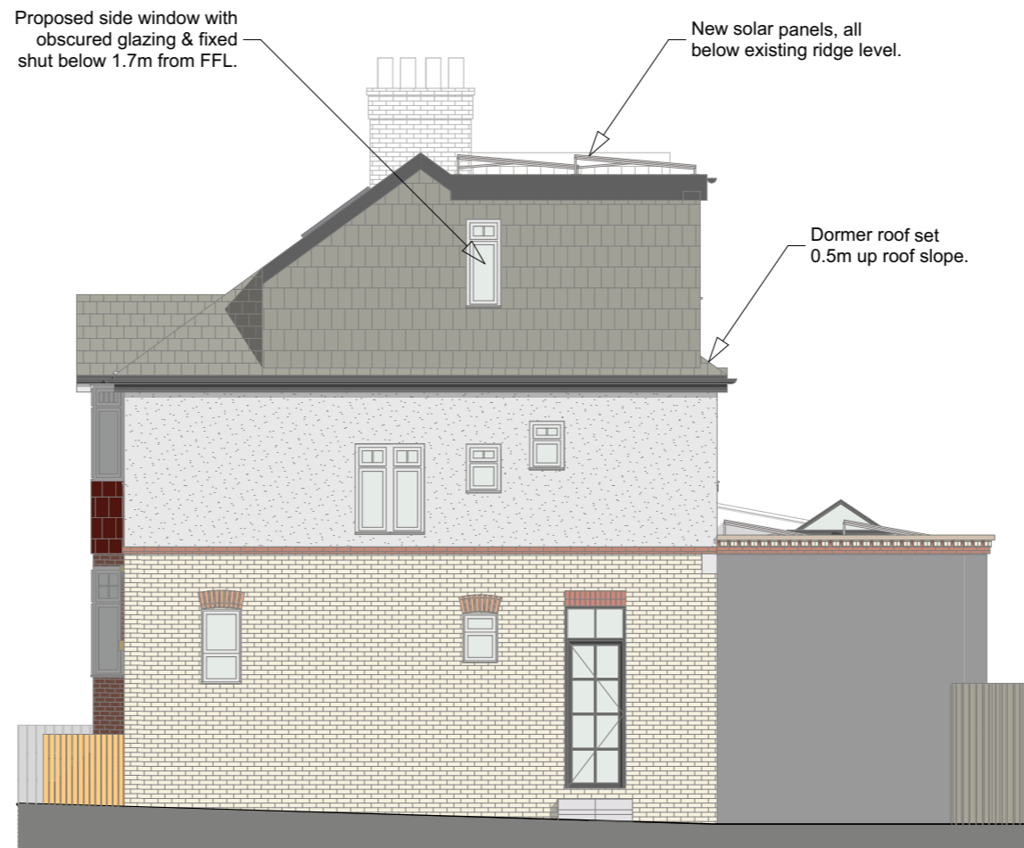
South West Elevation
