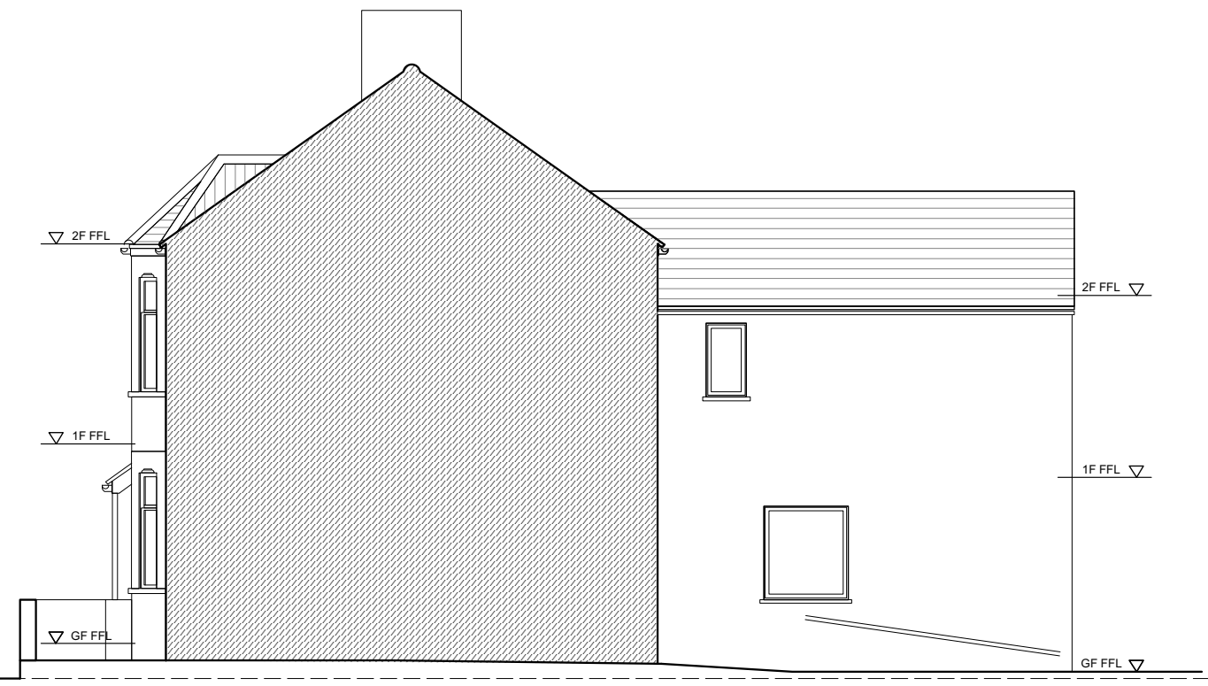
03 Existing Side Elevation 1:100 @ A3
