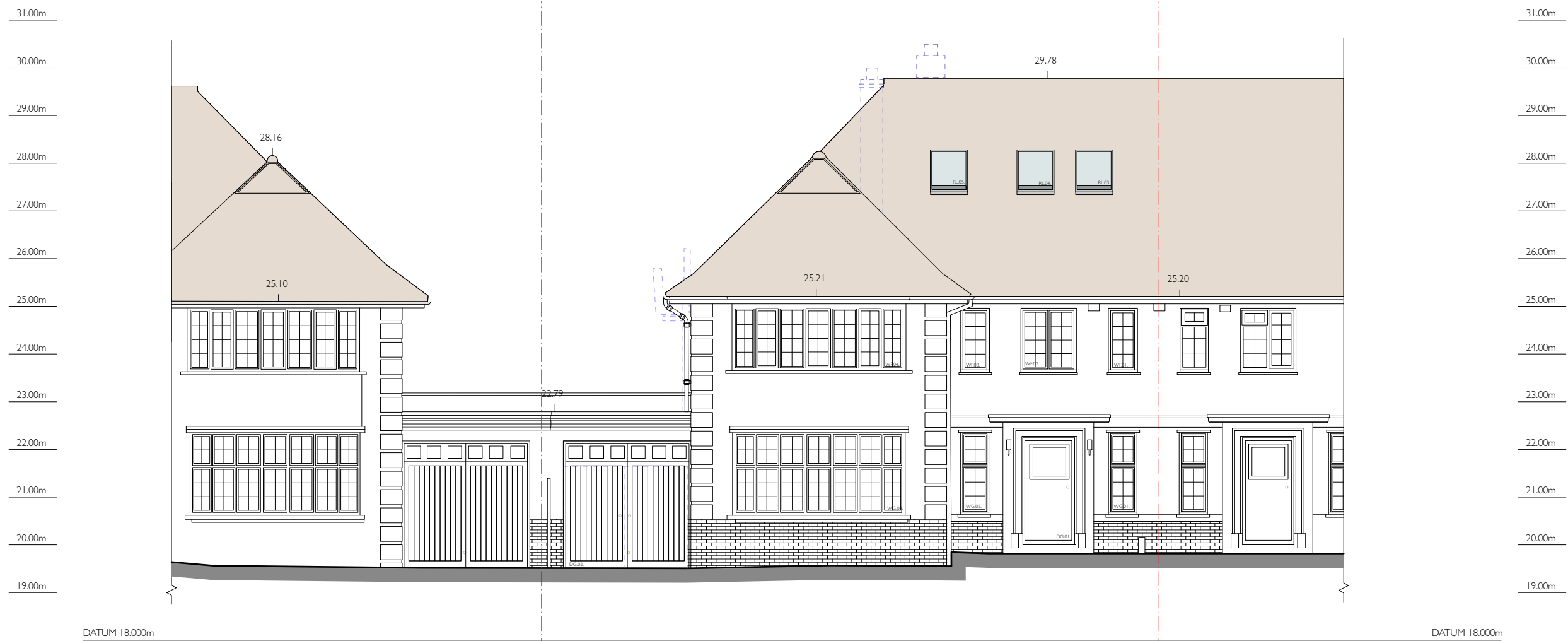
FRONT ELEVATION
