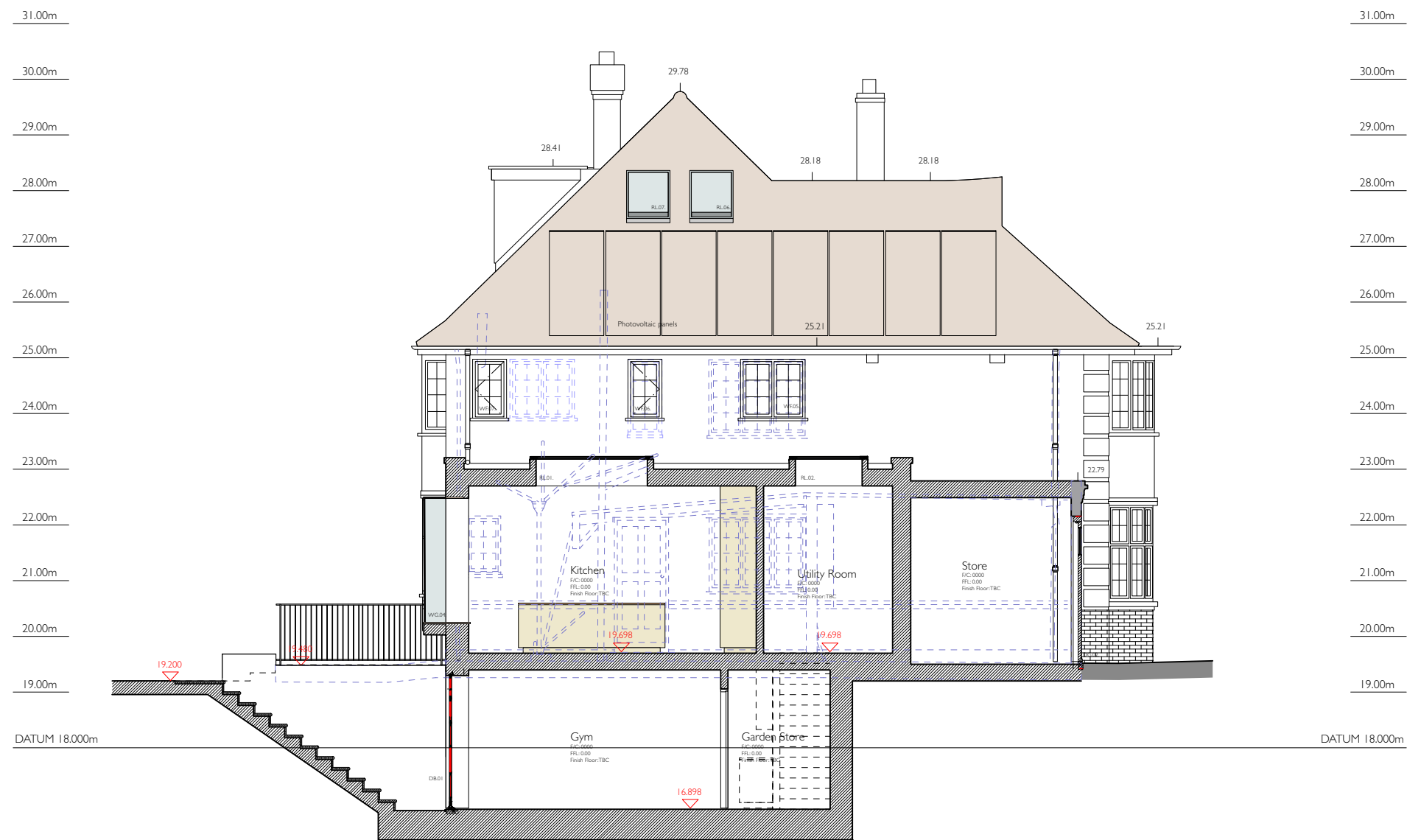
SIDE ELEVATION
