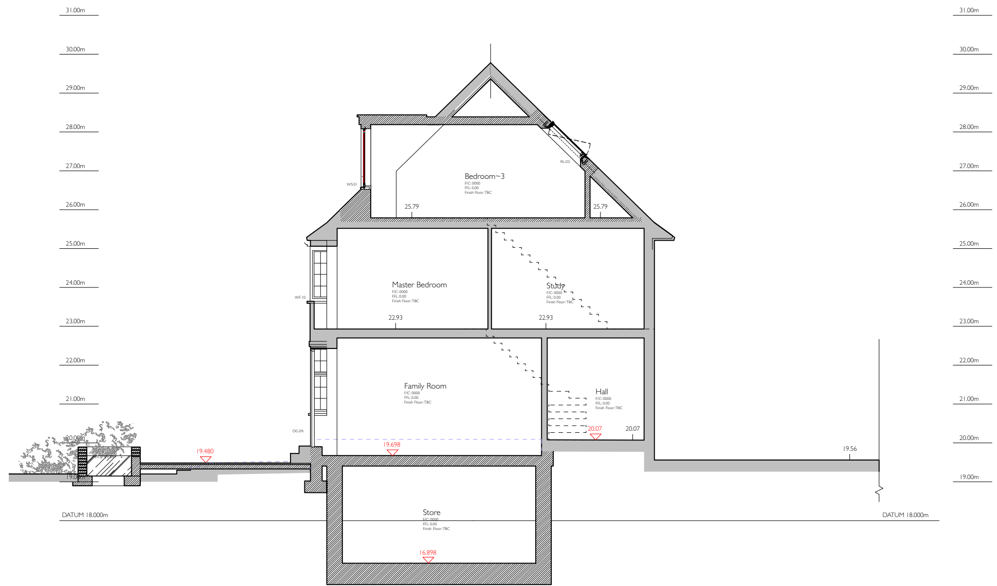
SECTION B-B
