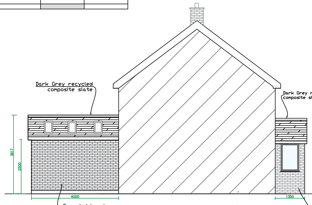
Proposed Side (East) Elevation
