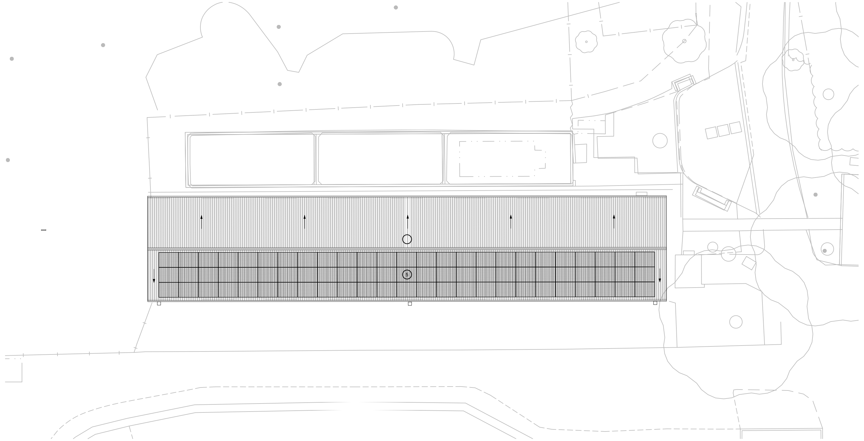
1 / Tractor Shed - Proposed Roof Plan 1:200
